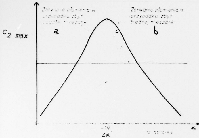
Fig. 5. Characteristics of the operational stability of the combustion chamber: C_2 \max - maximum speed in the intake section of the combustion chamber; \alpha - excess air number in the combustion zone of the chamber; \Delta \alpha - range of stable combustion. Legend: a) Flameout when the mixture is too rich; b) flameout when the mixture is too poor
