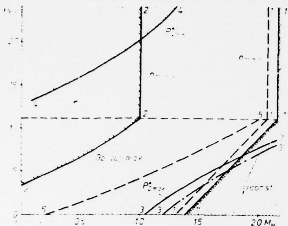
Fig. 1. Regions of possible limitations in the operational range of turbojet engines: line 1'-1' - limitation due to T_H^* \max ; 1-1 - limitation due to the range of stable operation of the compressor, on line 1-1 n_{ZR} = n_{ZR} \min ; 2-2 - limitation due to n_{ZR} = n_{ZR} \max ; 3-3 - beginning of limitations due to durability, governed by the pressure behind the compressor P_2^* = P_2^* \max ; 3'-3' - limitation due to the dynamic thrust q_{\max} = (k/2)P_H M ; 4-4 - limitation of the possibility of using the afterburner due to minimum pressure of the gases behind the turbine P_4^*
