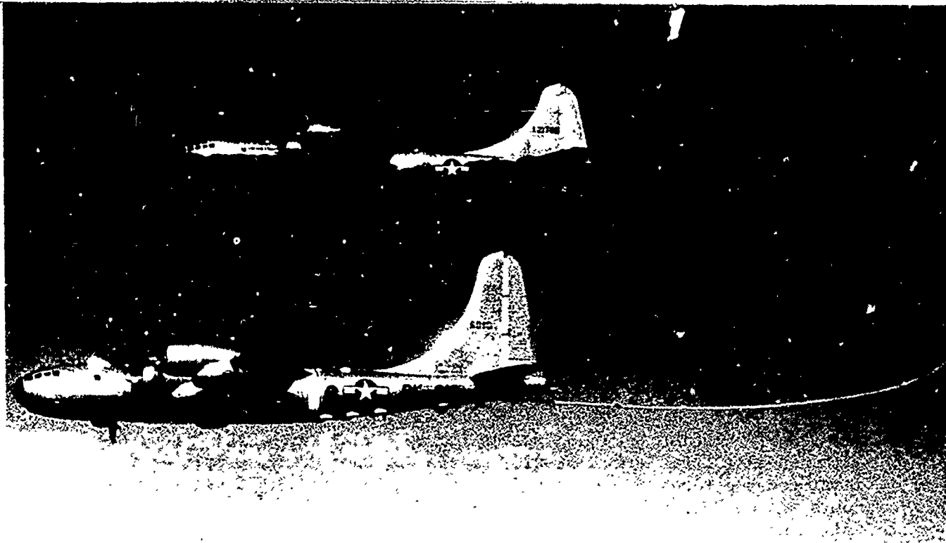
B-50 being refueled by KB-29M tanker
