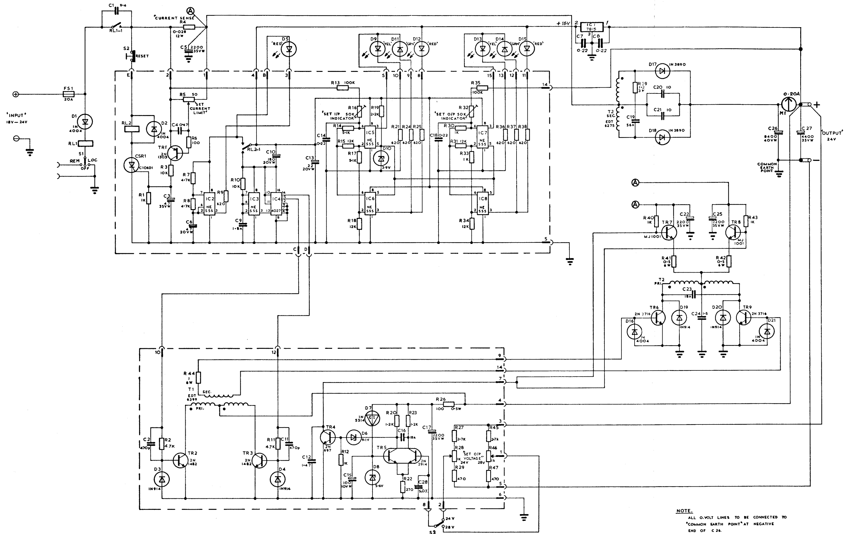
Figure 4. Circuit diagram
