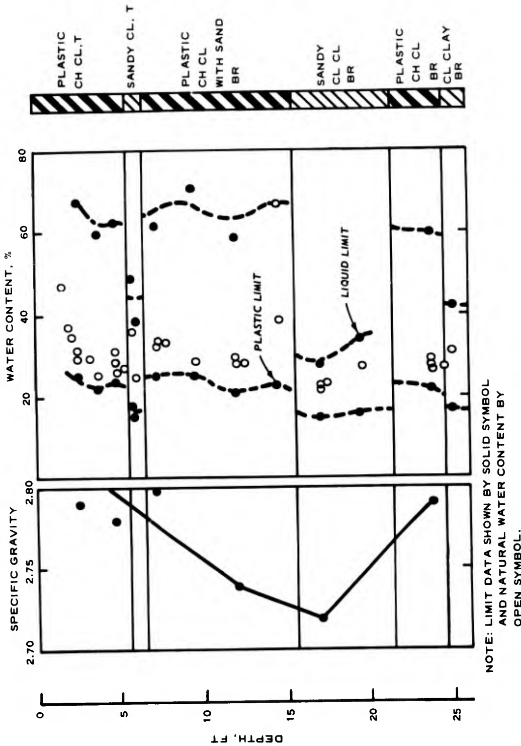
Figure 13. Classification of boring samples taken November 1976, Sigonella test site
