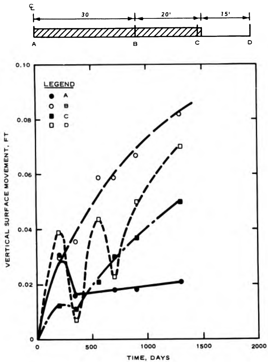
Figure 21. Vertical surface movement with time at the Fort Carson test site
