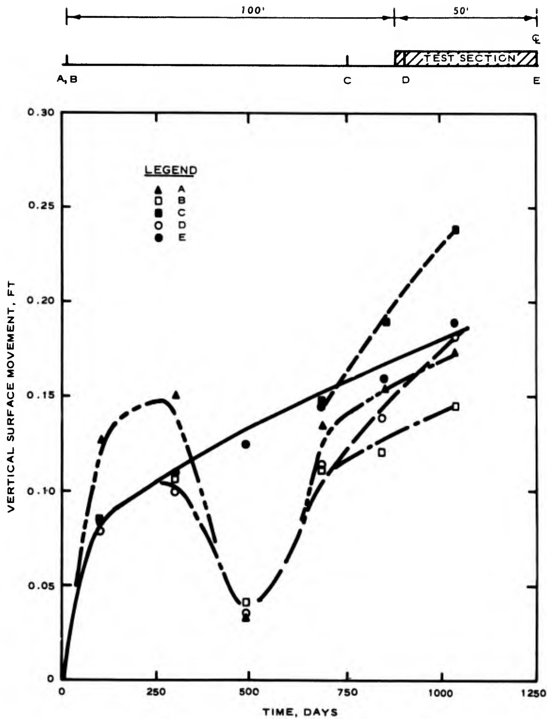
Figure 18. Vertical surface movement with time at the Lackland test site
