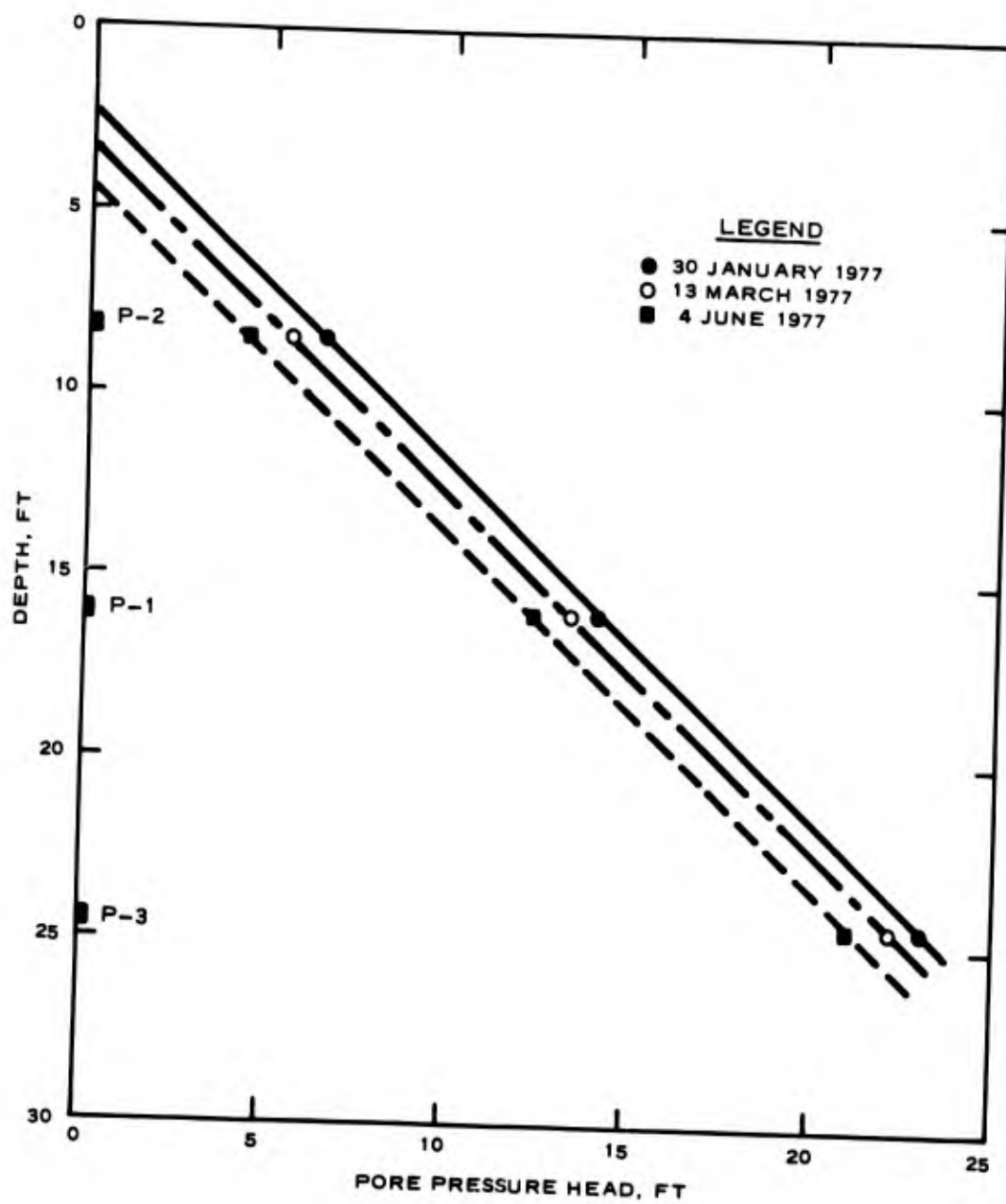
Figure 24. Profile of the pore pressure head at the Sigonella test site
