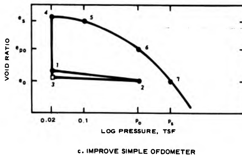
Figure 26. Schematic diagrams of void ratio - log pressure relationships of three types of swell tests
