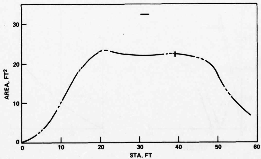
Figure 9 - Lift/Cruise Effect on Aerodynamic Lines
