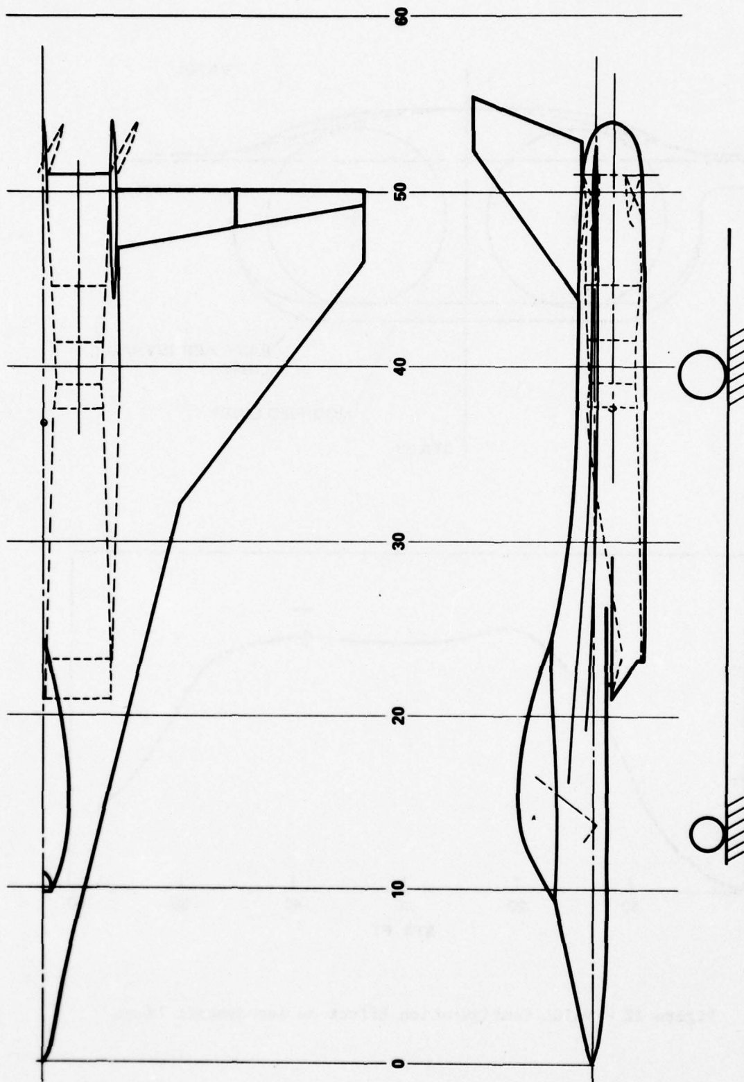
Figure 11 - VATOL Configuration
