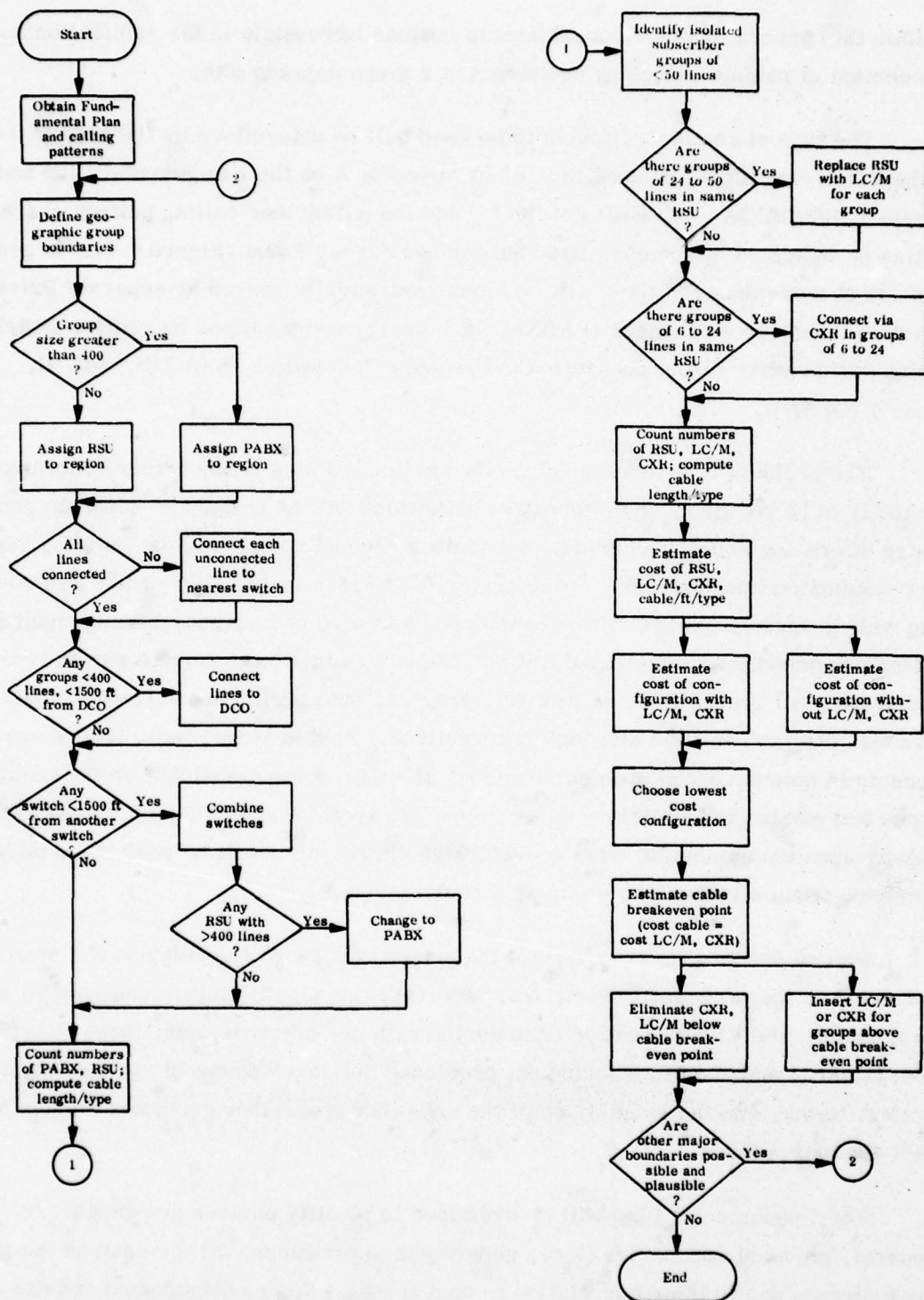
Figure 5-2. Functional Flow, Switching Scheme Development Guide
