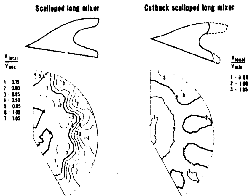
Figure 5-24 Effect of Lobe Cutback on Tailpipe Exit Velocity Contour Map of Long Flowpath Mixer Scalloped (without Engine Secondary Flow Simulation)
