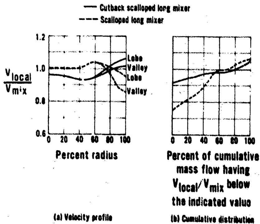
Figure 5-25 Effect of Lobe Cutback on Tailpipe Exit Velocity Profile and Cumulative Mass Flow Distribution of Scalloped Long Flowpath Mixer (without Engine Secondary Flow Simulation)
