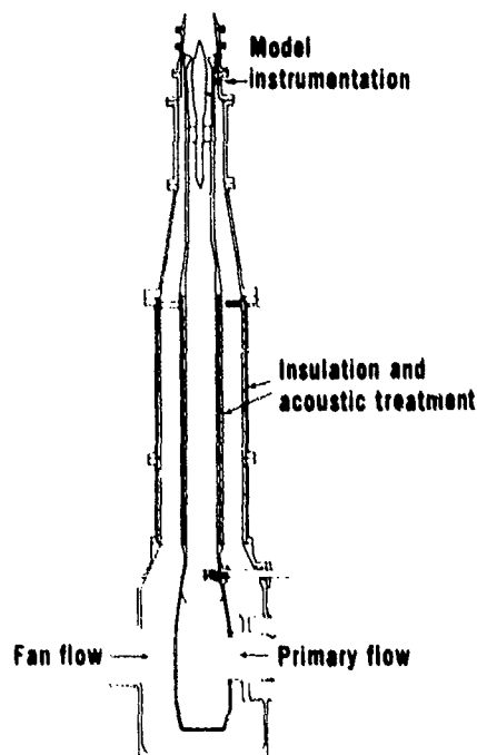
Figure 3-3 Exhaust System Test Installation
