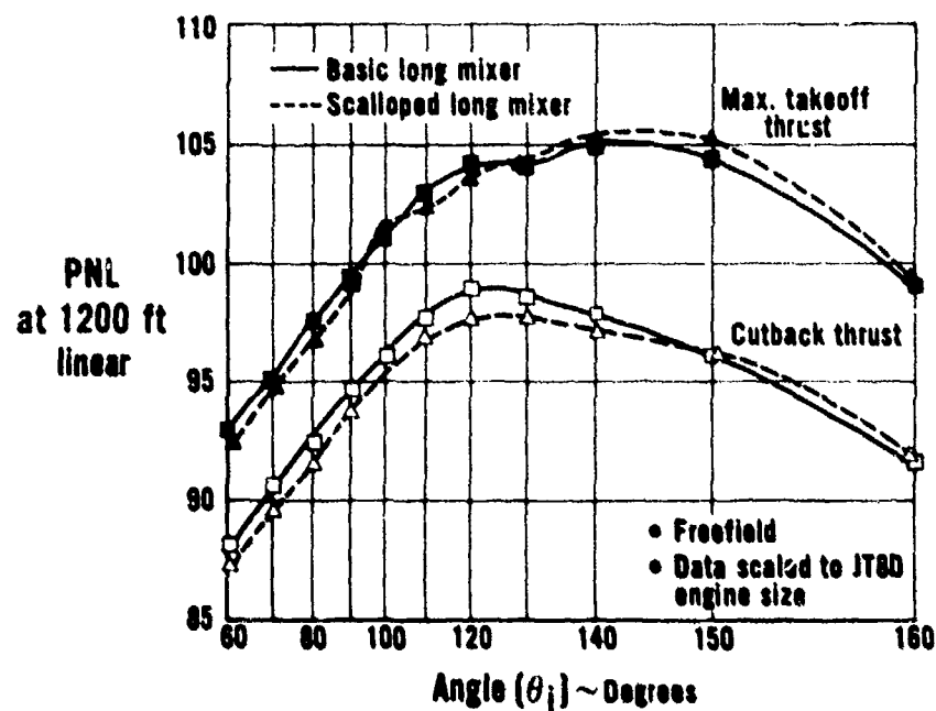
Figure 5-20 Effect of Scallop on Perceived Noise Level Directivity of Long Flowpath Mixer (without Engine Secondary Flow Simulation)
