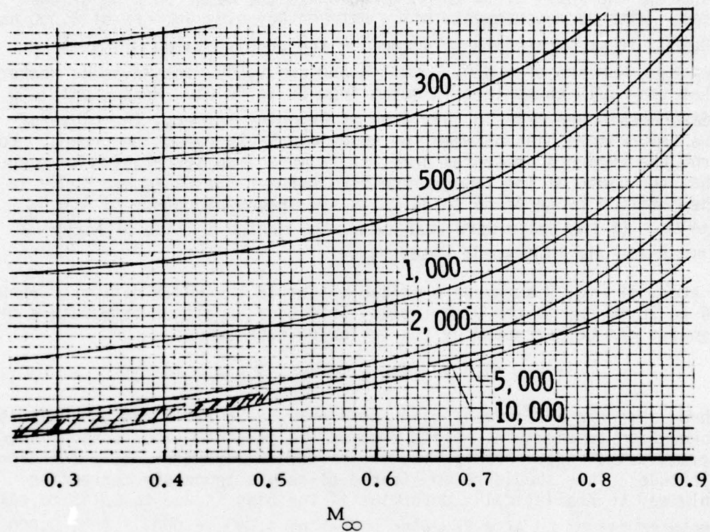
Figure 5. Values of C_d vs. Mach Number for Given Reynolds Number taken from Bailey and Hiatt
