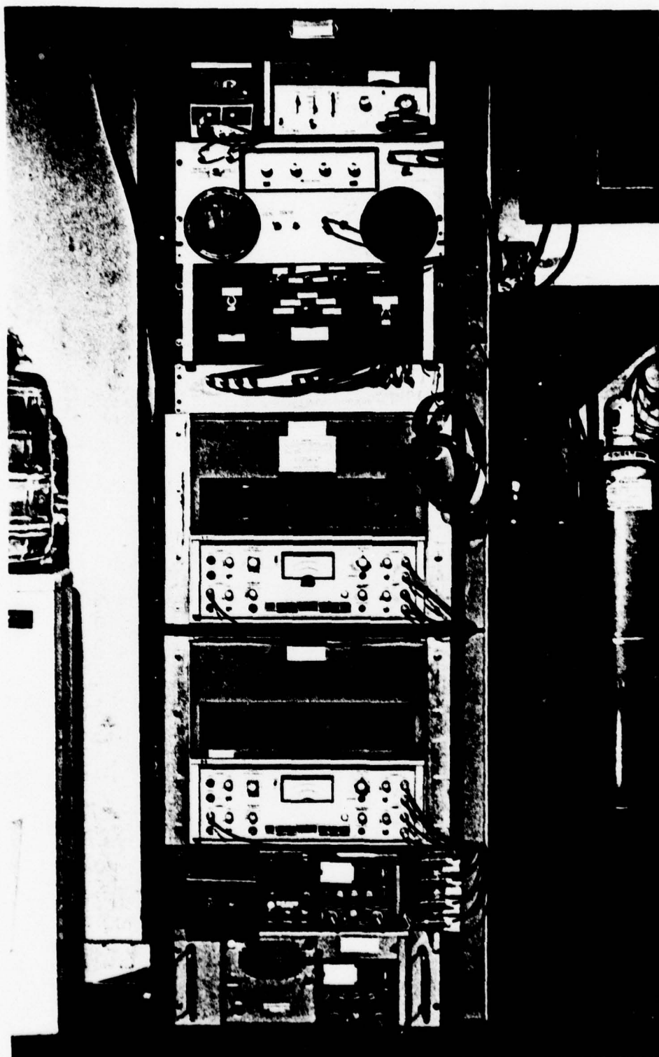
Figure 2-5. Receiving equipment at Texas Tech antenna site in Lubbock.
