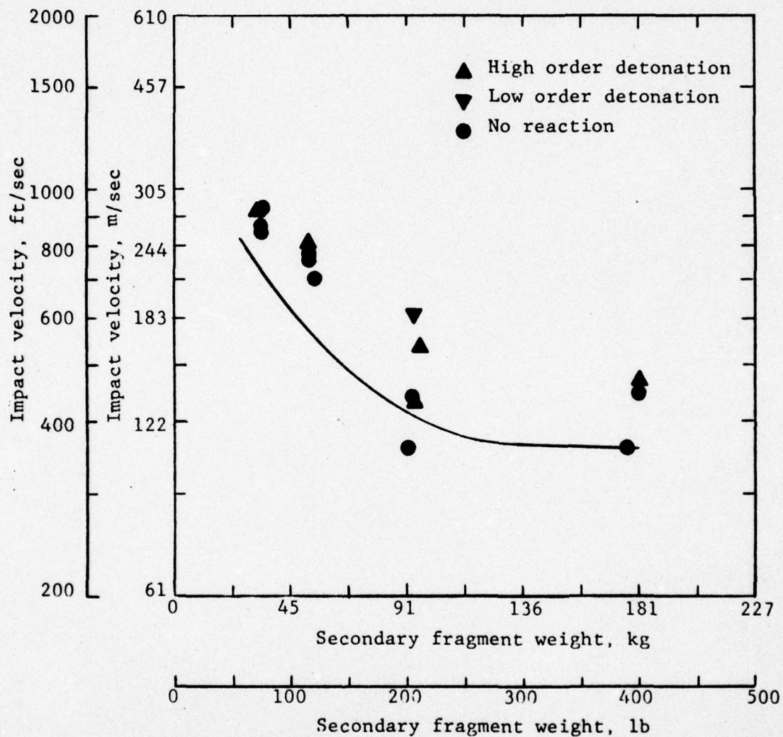
Fig 18 Secondary fragment impact results for 81 mm (1362A1) mortar shell, "just filled" condition with Composition B at 64-88°C (143-190°F). Data in Appendix, table 7.
