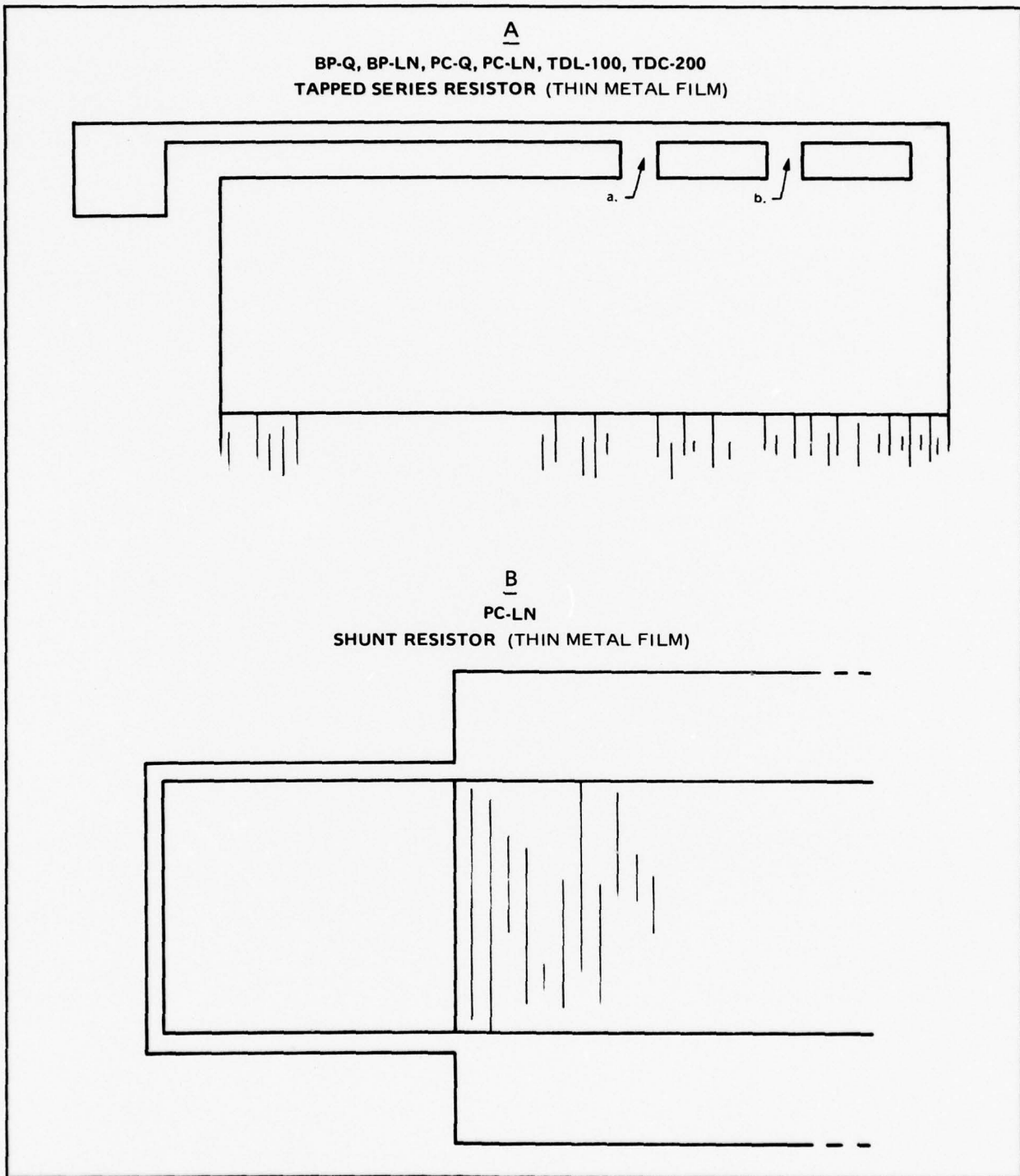
Figure 2.2-3. Resistor Detail
