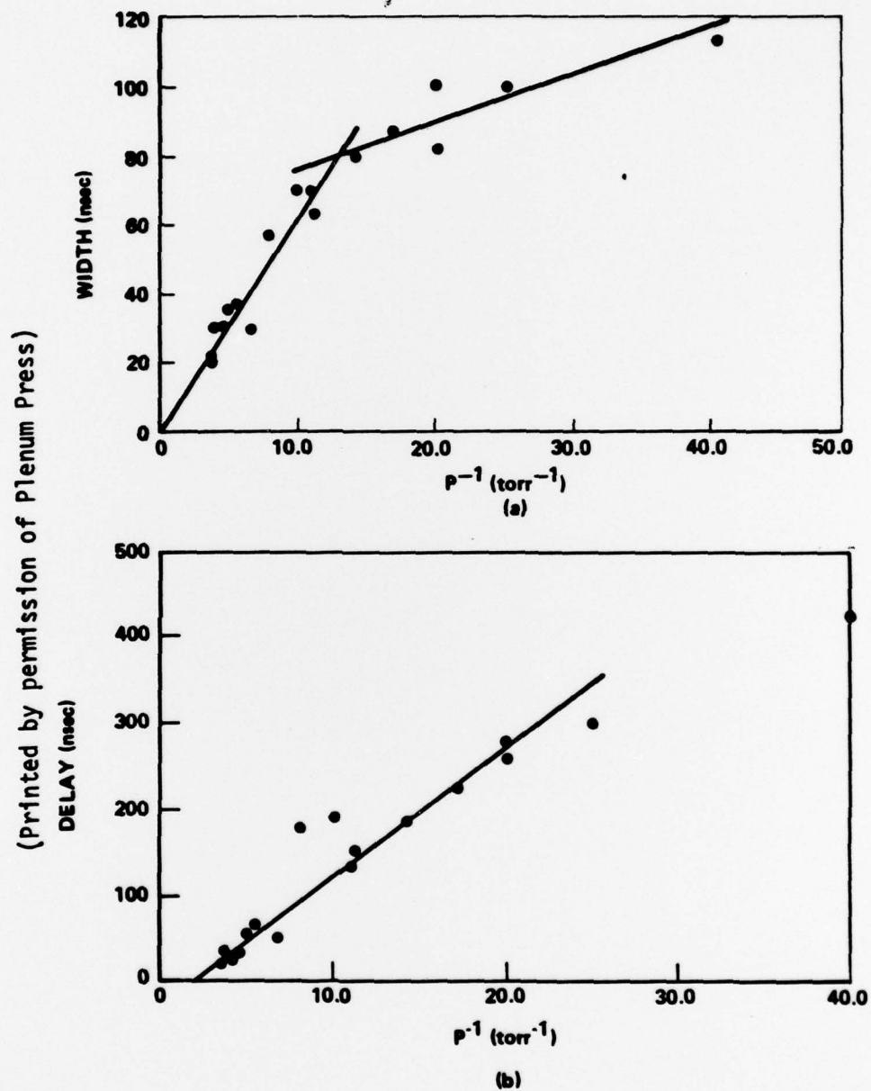
Figure 4. FIR Width and Delay vs Inverse Pressure p^{-1} .
