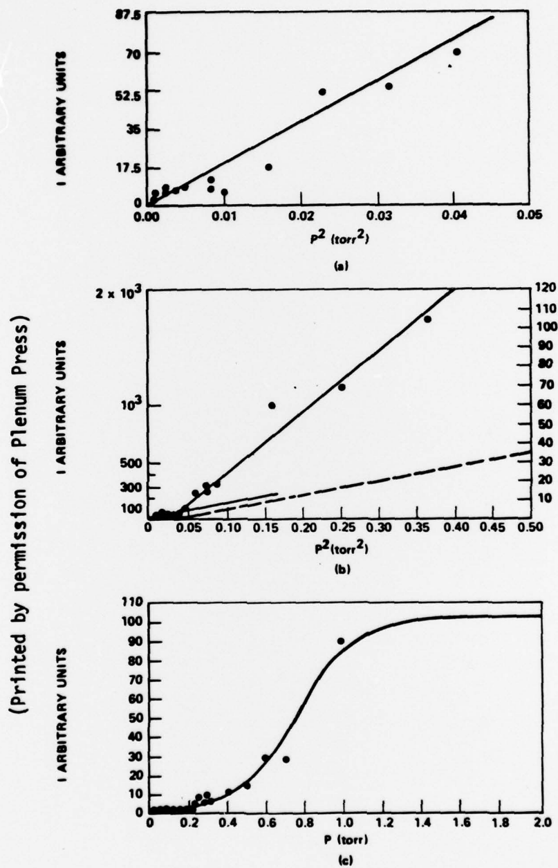
Figure 3. FIR Intensity I as a Function of Pressure P .
