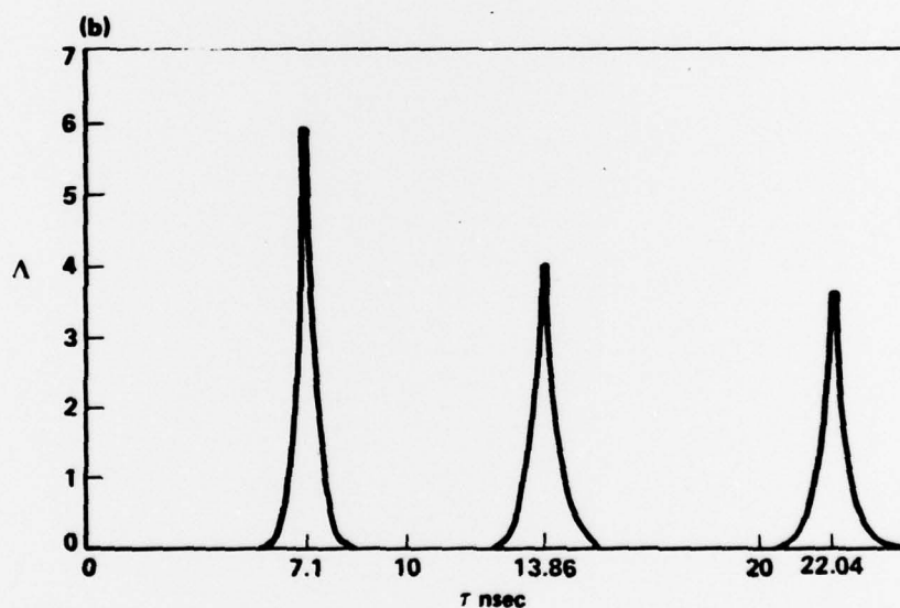
Figure 6(a) Model Energy Level Scheme; (b) Calculated FIR Pulse Sequence Evolution vs Time \tau from IR Pump Turn-on for a Step Function Pump Envelope.
