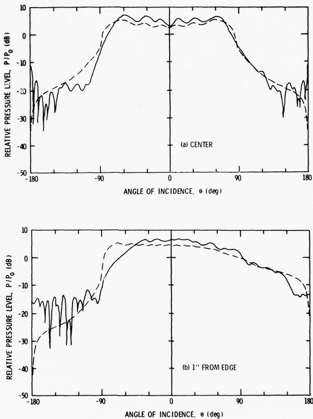
Figure 6.6 Experimental (solid line) and Theoretical (dashed line) Patterns for a Hydrophone on a Rigid End-Cap, Rigid Cylinder at 20 kHz.
