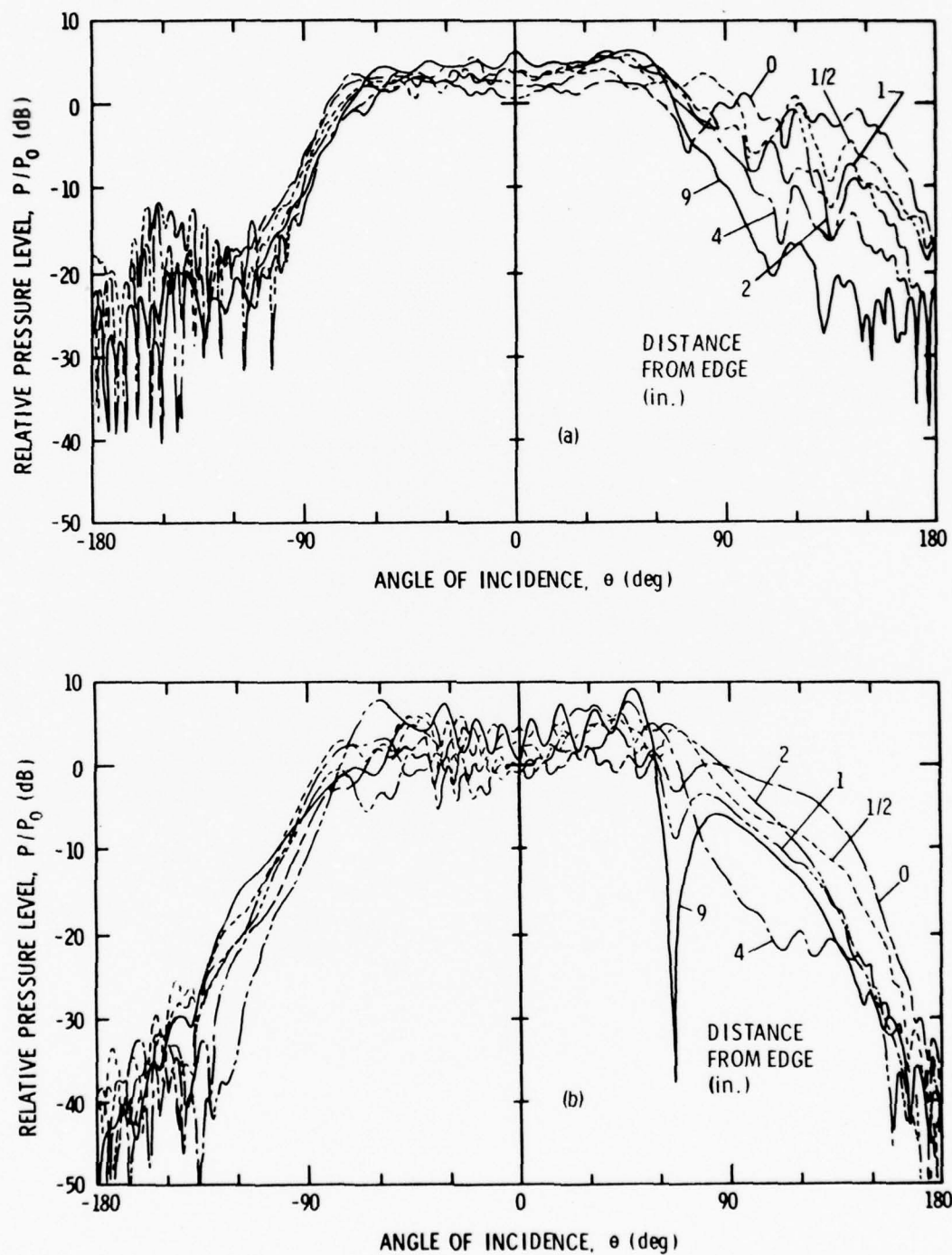
Figure 6.18 Patterns of a Hydrophone on a Rigid End-Cap with a Rigid (a) and a Soft (b) Cylinder at 30 kHz.
