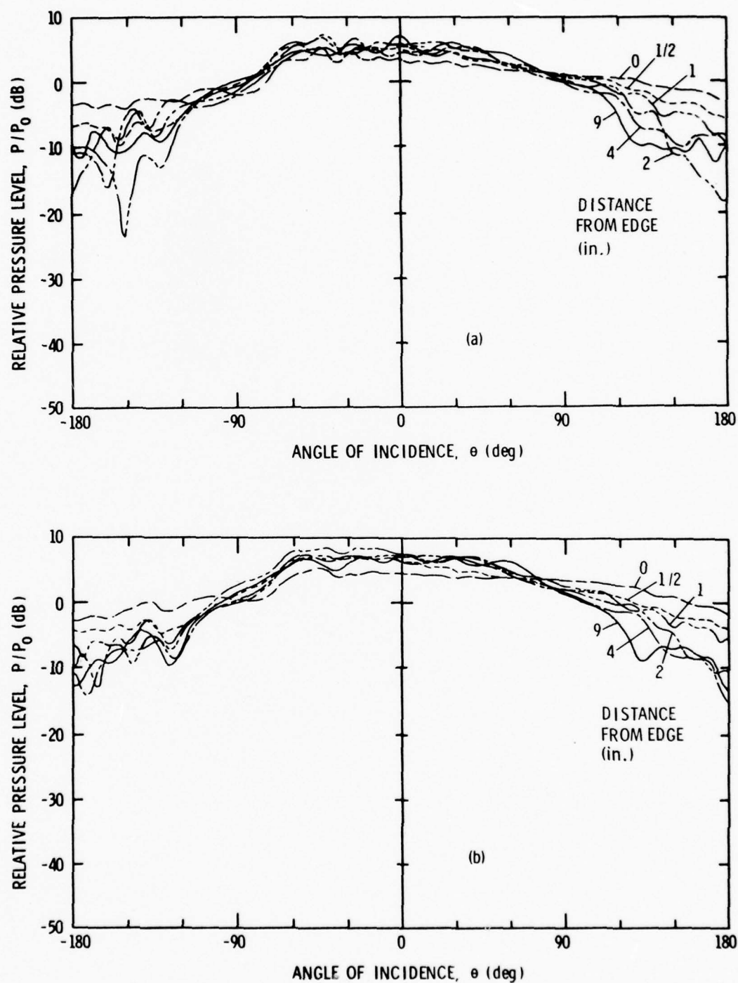
Figure 6.10 Patterns of a Hydrophone on a Rigid Disk (a) and a Rigid Square (b) at 15 kHz.
