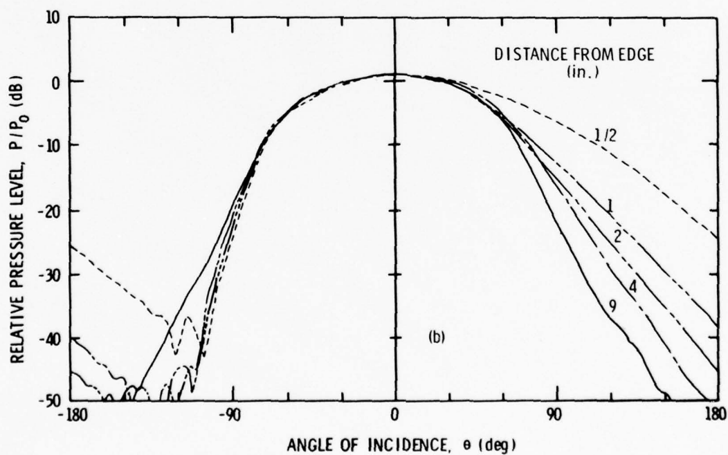
Figure 6.14 Patterns of a Hydrophone on a Soft Disk (a) and a Soft Square (b) at 20 kHz.
