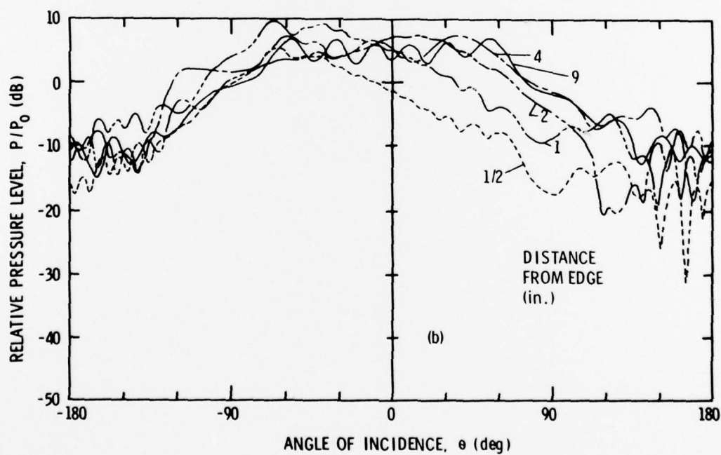
Figure 6.24 Patterns of a Hydrophone on a Rigid Disk (a) and a Rigid Square (b) with a Soft Scattering Bar at 20 kHz.
