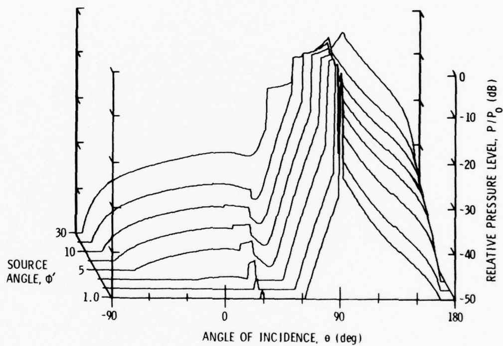
Figure 2.10 Calculated Directivity Patterns with Both Surface Impedance Ratios Equal to Z/\rho c = 1.5 as a Function of Source Angle.
