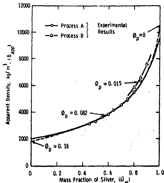
FIGURE 1. Apparent brush density for silver-graphite brushes, with fractional porosity ( \theta_p ) as indicated.
