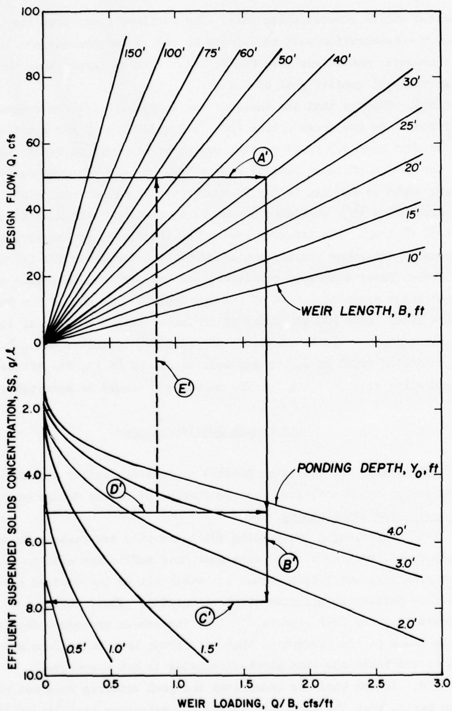
Figure 28. Example Problem 2 (part 2)
