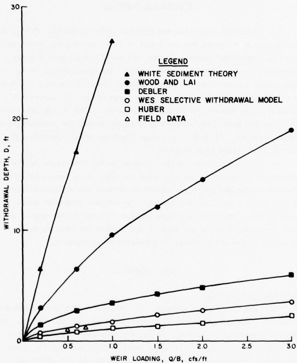
Figure 18. Comparison of withdrawal depth models for Fowl River dredged material
