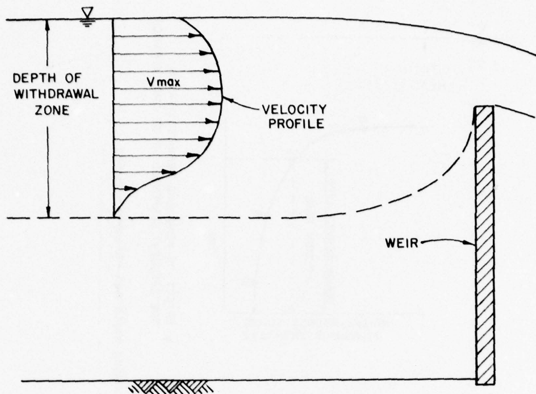
Figure 3. Withdrawal depth and velocity profile
