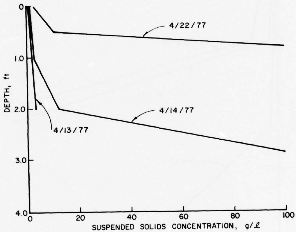
Figure 15. Effect of time on suspended solids concentration profile for Fowl River site near the weir
