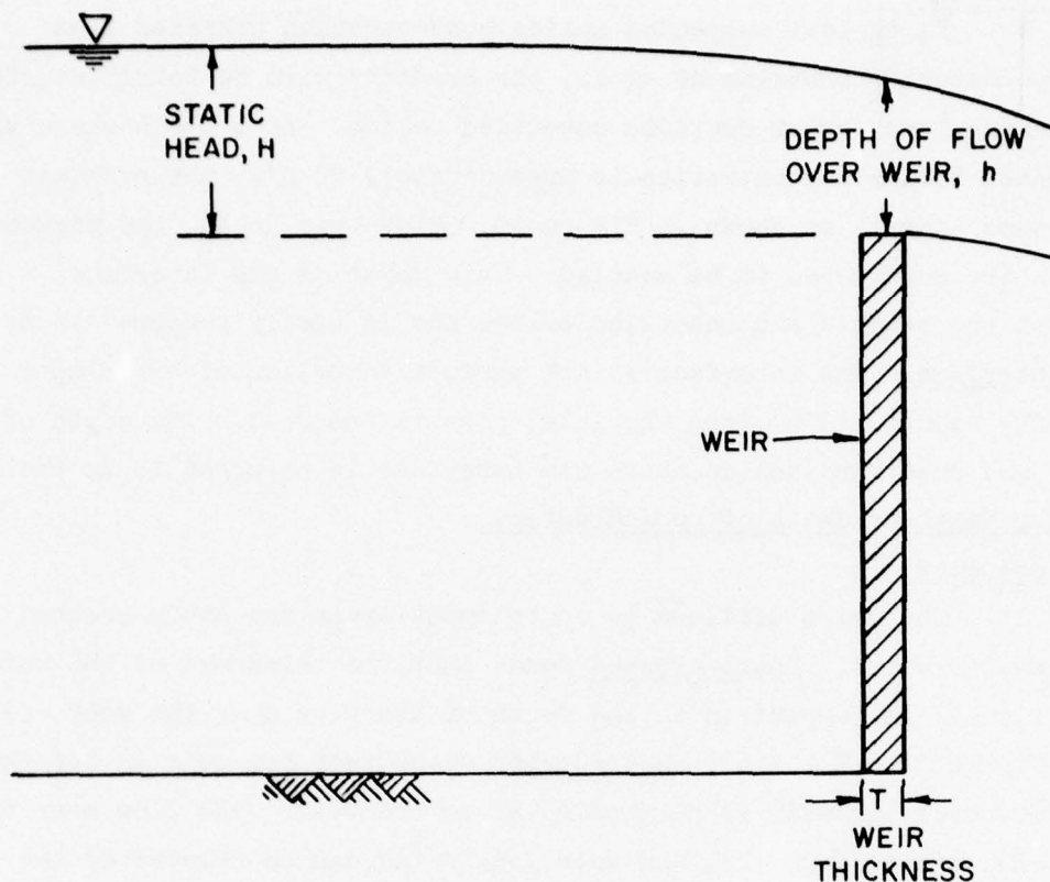
Figure 2. Weir characteristics
