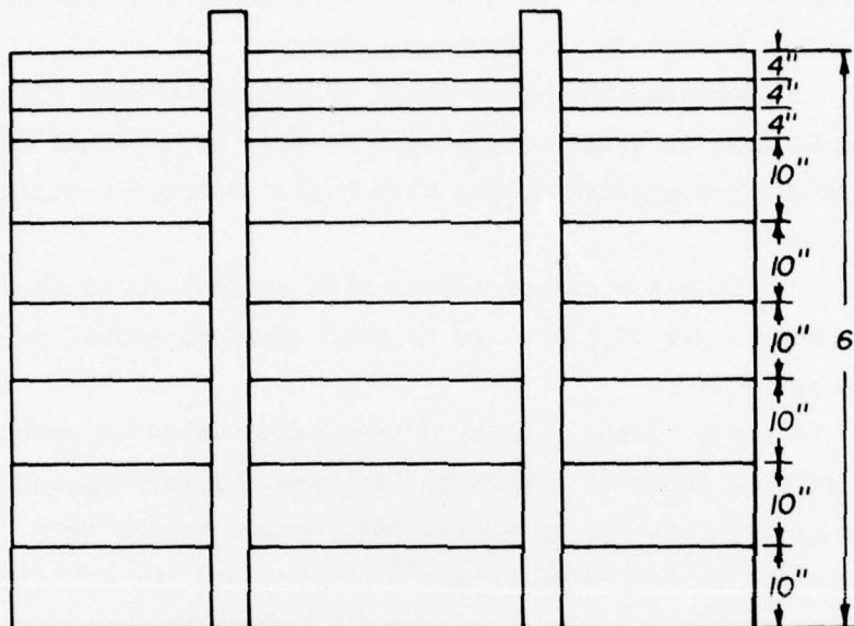
Figure 32. Suggested weir boarding
