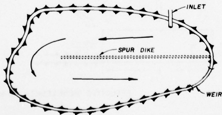
Figure 31. Short-circuiting and dead zones
