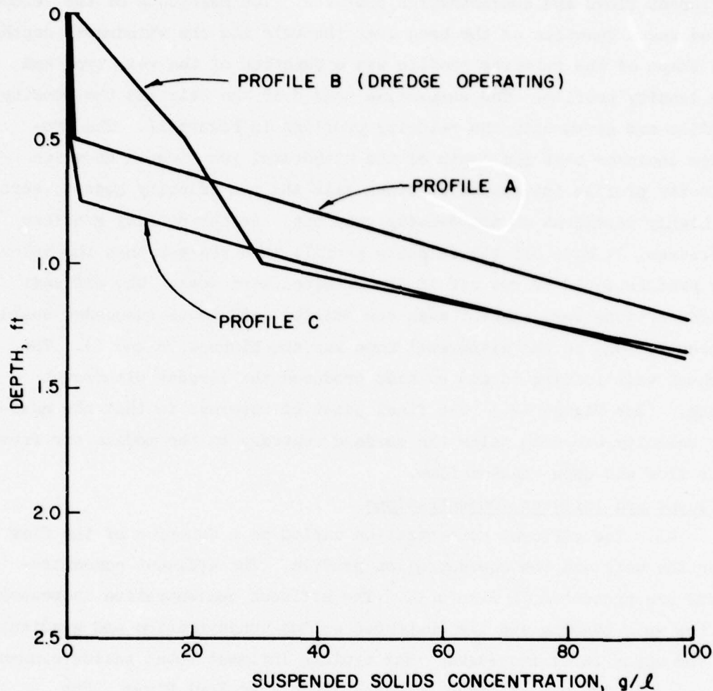
Figure 16. Effect of short-circuiting on suspended solids concentration profiles for Oyster Bay site near the weir
