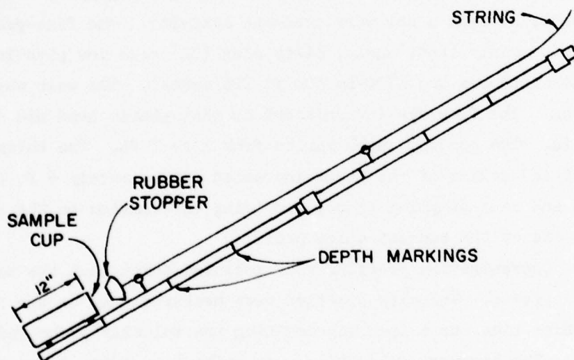
Figure 9. Sediment sampler
