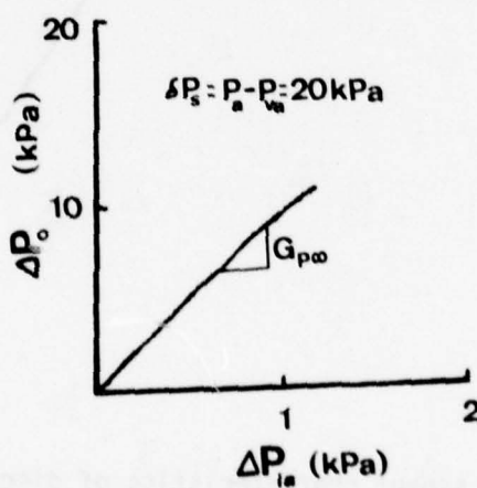
Figure 27. Amplifier transfer characteristics (experimental, infinite load impedance).
