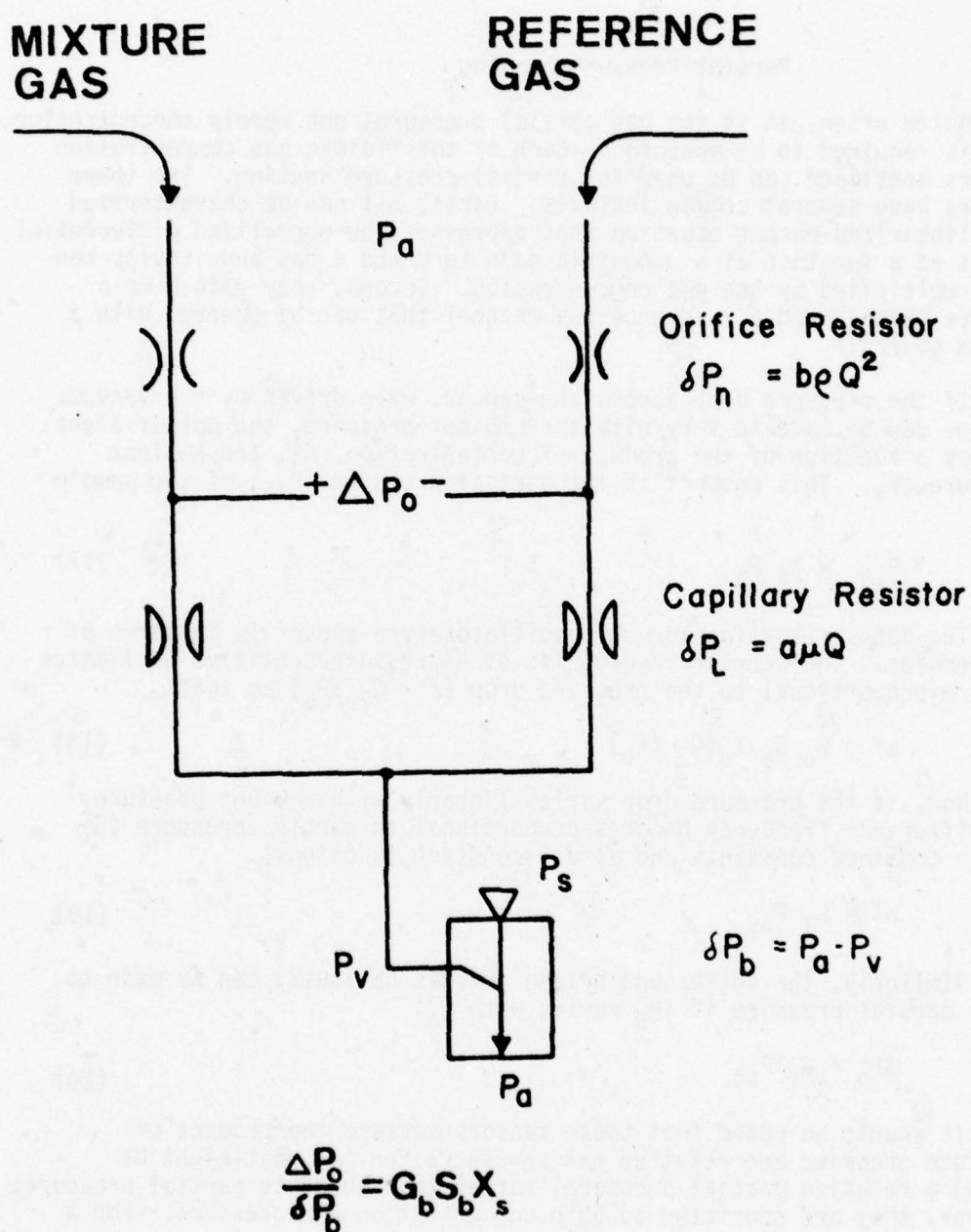
Figure 4. Bridge-type gas concentration sensor.
