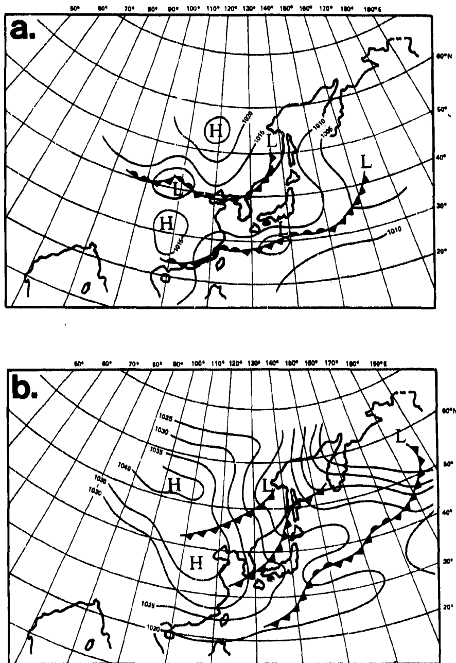
Figure 4-3. Approaching system/front: (a) approaching secondary or trailing low pressure system and (b) approaching secondary cold front.
