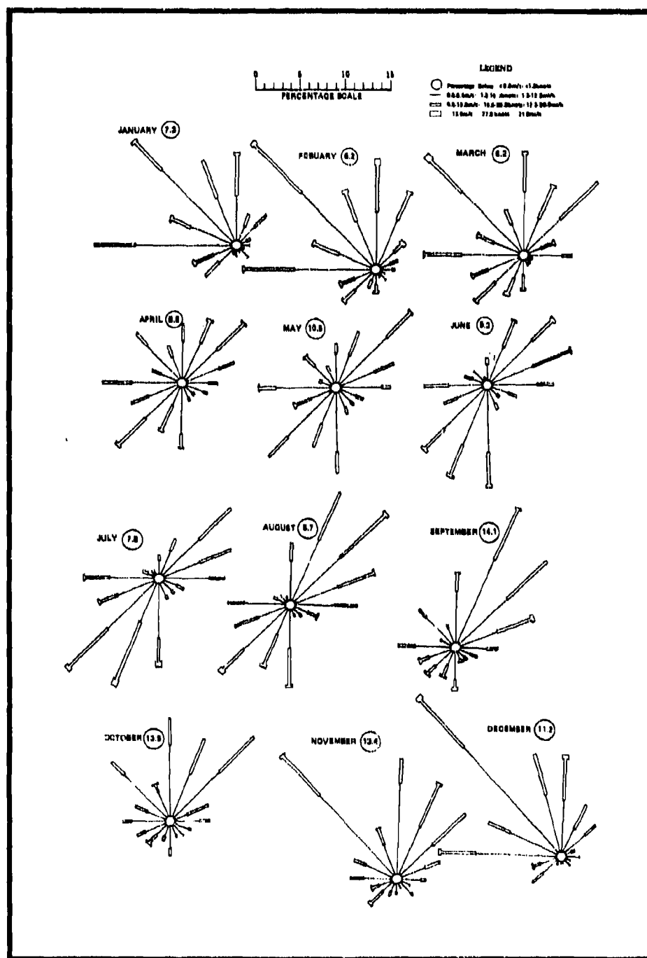
Figure 5-9. Monthly wind roses for the Pusan area (from Climatic Atlas of Korea, 1962).
