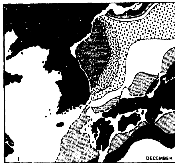
Figure C-12. Thermocline data for December.
