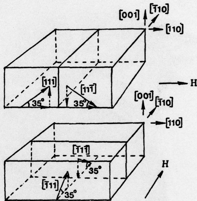
FIGURE 5 MODEL OF 71^\circ WALLS OBSERVED IN A \text{TbFe}_2 SINGLE CRYSTAL (100) SURFACE.
