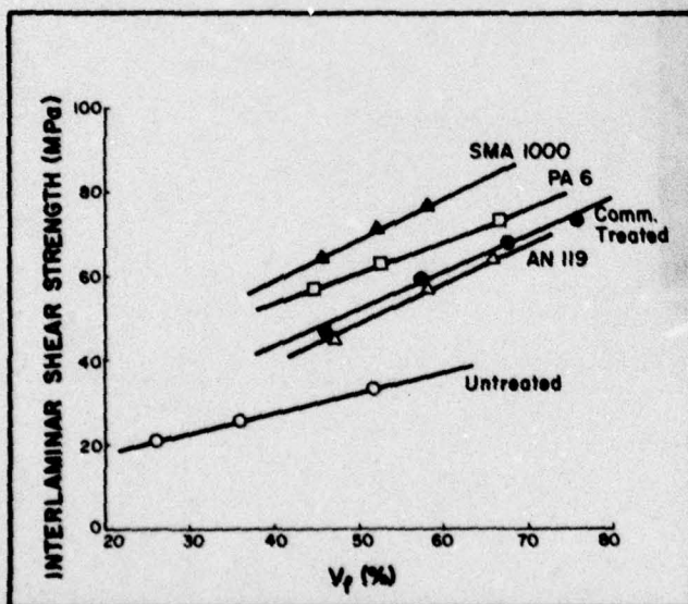
Figure 5. Interlaminar shear strengths of composites prepared from CG-3 graphite fibers electrodecoated by the indicated copolymers.
