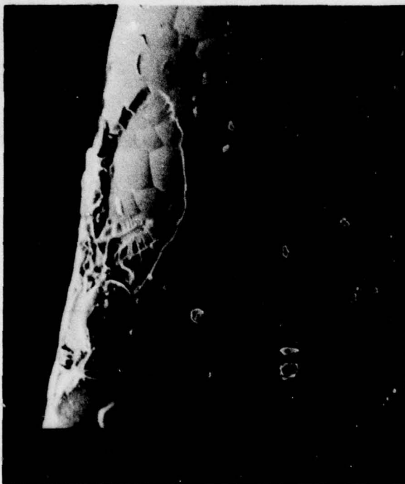
Figure 9. SEM of Boron fiber electrocoated by styrene-maleic anhydride copolymer.
