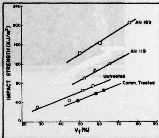
Figure 6. Impact strengths of composites prepared from CG-3 graphite fibers electrodecoated by the indicated copolymers.
