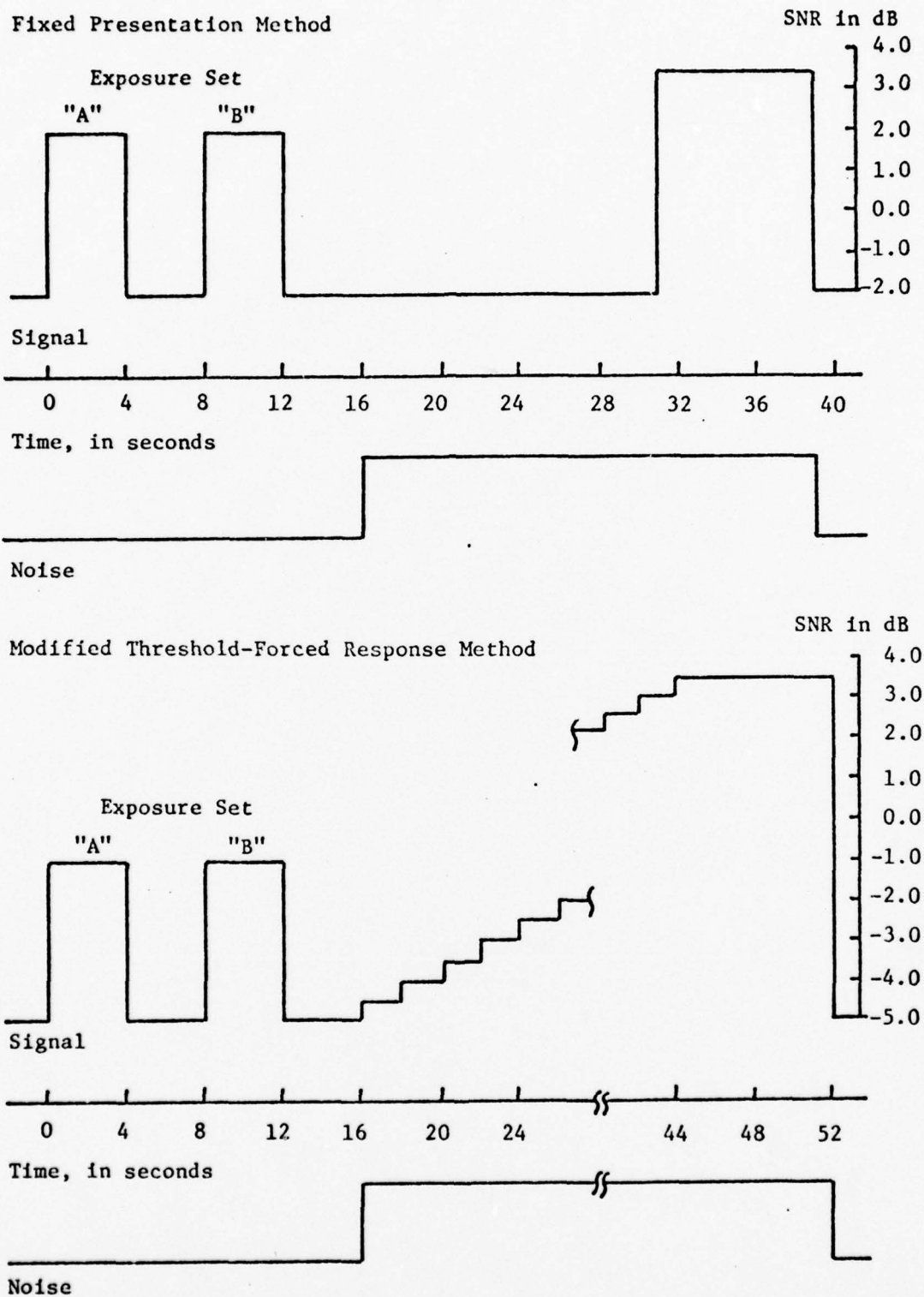
Figure 1. Fixed Presentation and Modified Threshold-Forced Response Paradigms
