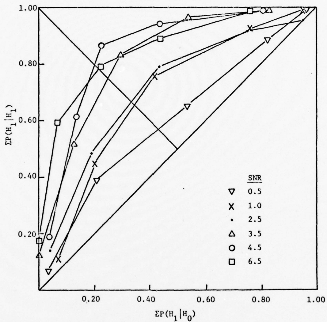
Figure 5. ROC Using the MTFR Method
