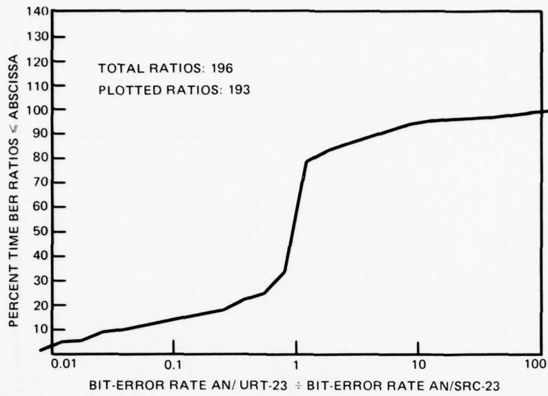
Figure 30. All-frequencies cumulative distribution of ratios of adjacent bit-error rates at the ship.
