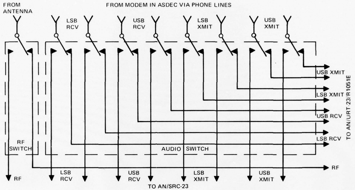
Figure 5. Audio and rf switch panel arrangements.
