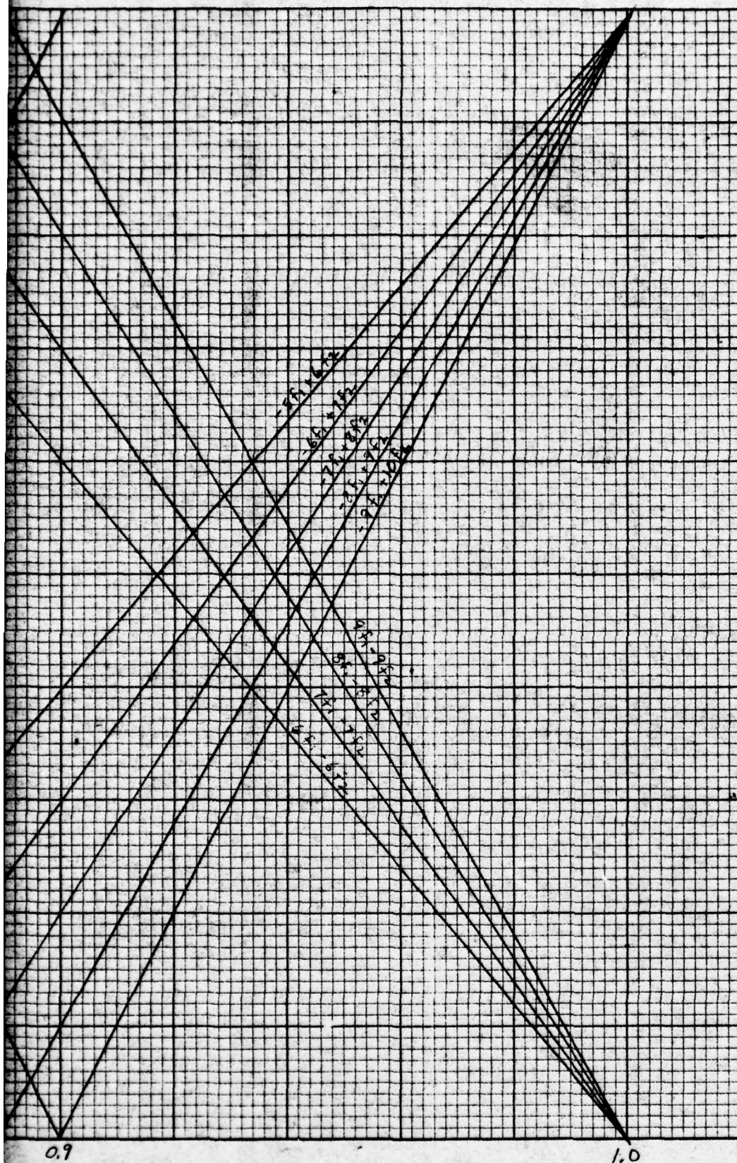
Figure A-2 INTERMODULATION CHART Order: 11-19
