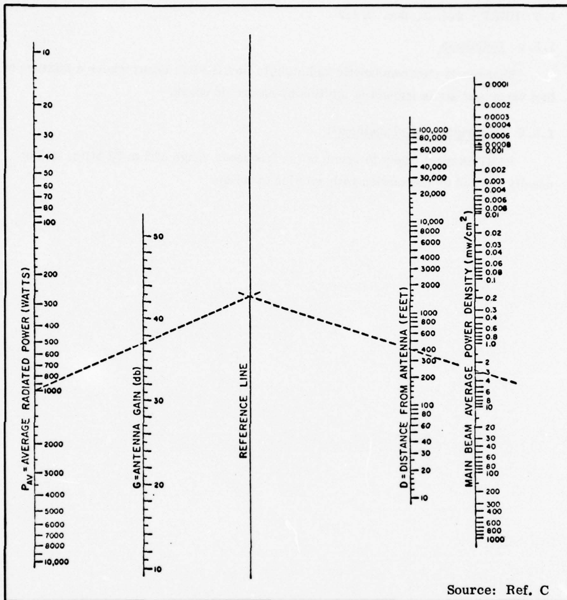
Figure 1-3. Power Density Nomograph
