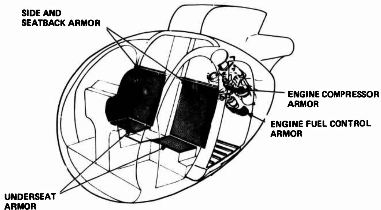
Figure 26. Armor Kit
