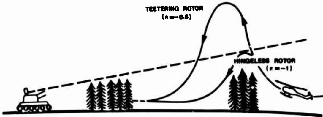
FIGURE 14: TYPICAL COMPOUND MANEUVER
