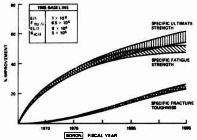
Fig. 33 Materials properties improvement and use goals.
