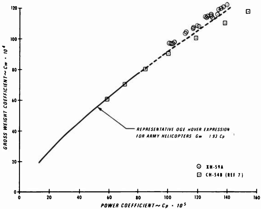
Fig.6 XH-59A and current army helicopters
