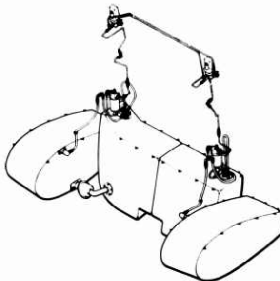
Figure 16. Fuel System.
