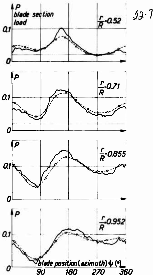
Fig. 13 - Evolution of local loads in the case of a moderately loaded 3-blade rotor ( \bar{L} = 16.1 ; \bar{D} = -2.3 ) at \mu = 0.3 ( \alpha_0 = -16^\circ ; \theta = 11.7^\circ ). Tests in S1-MA wind tunnel.
