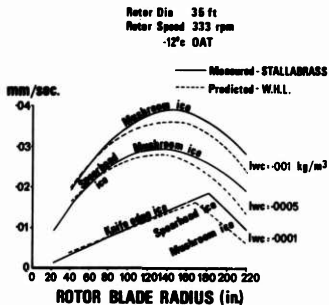
Fig.14 Comparison of Theory and Experiment for Ice Accretion
