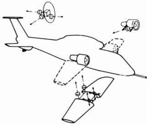
Figure 4.- RSRA Auxillary Measurements System.
