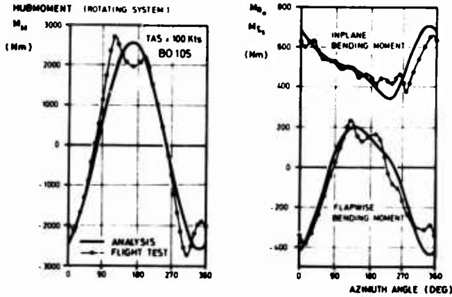
Fig. 7 Hub and Blade Root Moments in Forward Flight
