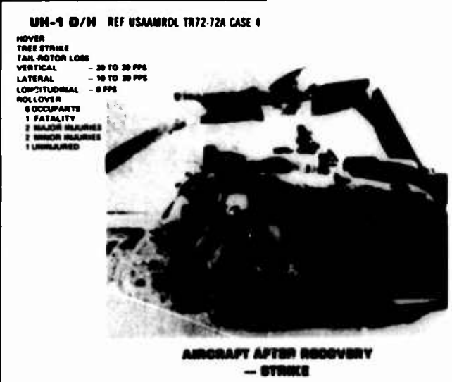
Figure 10. Comparison of Similar Accidents Involving Tail-Rotor Loss and Tree Strike; MIL-STD-1290 Crashworthiness Works
