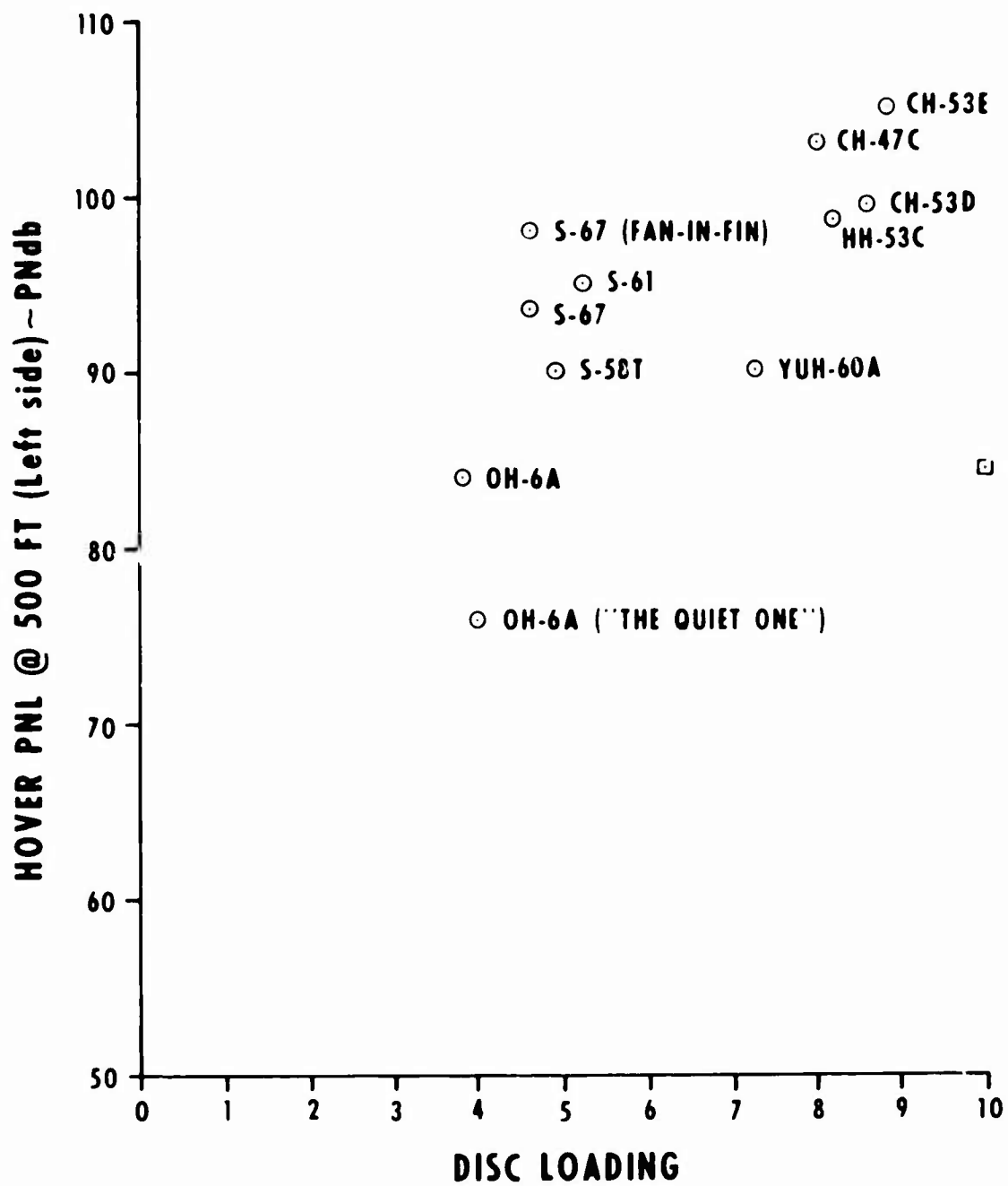
Fig.22 External noise hover
