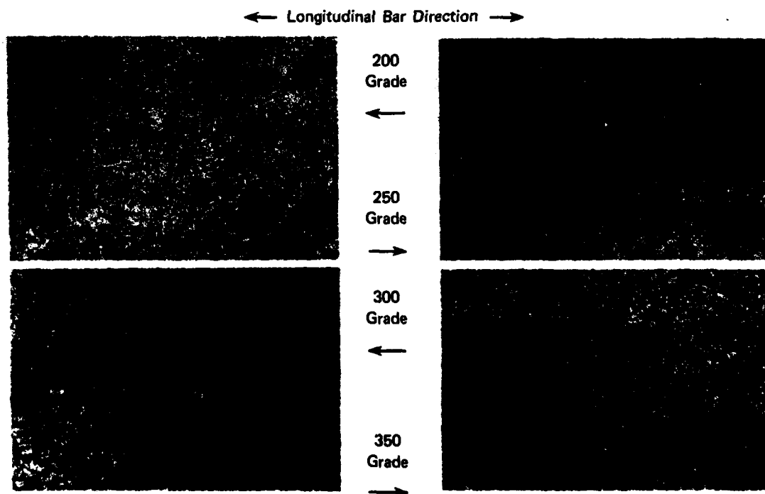
Figure 2. Microstructure of aged maraging steels. Mag. 250X (Maraging Etch: 5g \text{FeCl}_3 , 2 ml \text{HCL} , 296 ml \text{C}_2\text{H}_5\text{OH} )
