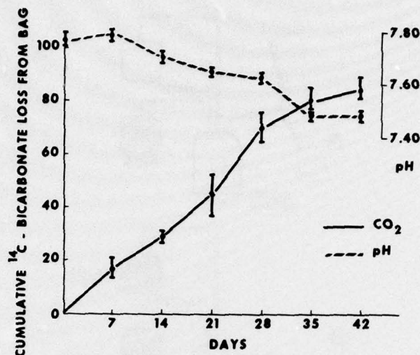
Fig. 2. The cumulative ^{14}\text{C} -bicarbonate loss per week in percent (—) and the change in pH (----) are both plotted against days. The amount of ^{14}\text{C} -bicarbonate lost is about 84.5 percent by 42 days, and the pH has dropped from 7.75 on day zero to 7.49 on day 42. This reveals the buffering ability of the bicarbonate system.
