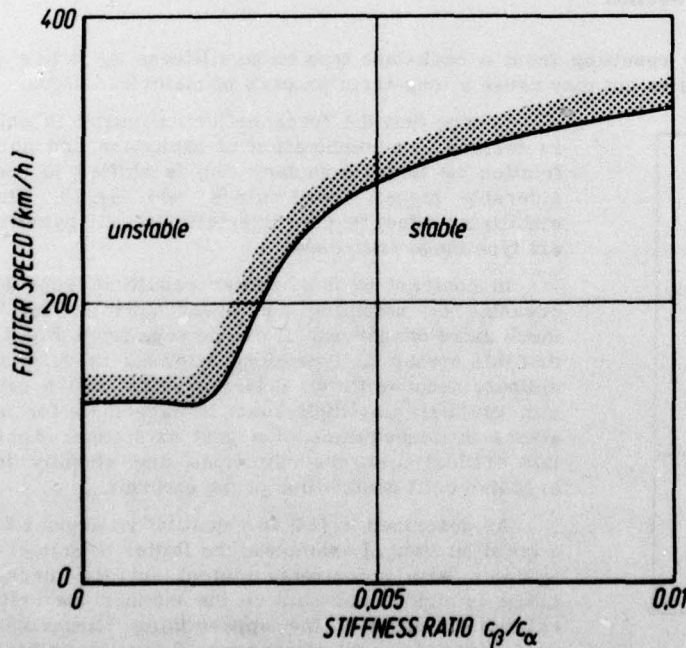
Fig. 15: Flutter speed of the "linearized" wing aileron section as function of changes of the linear hinge stiffness
