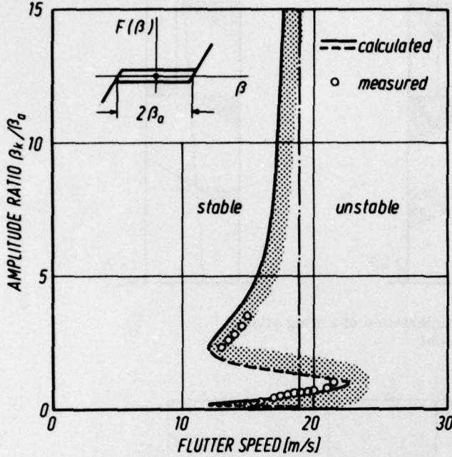
Fig. 19: Comparison of the measured and the calculated flutter boundary of the non-linear wind tunnel test model
