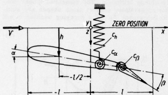
Fig. 11: Sketch of a wing aileron section with three degrees of freedom
