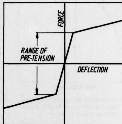
Fig. 6: Schematic force deflection diagram of a pre-tensed spring tab
