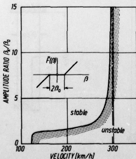
Fig. 12: Effect of back-lash on the flutter stability of a wing aileron section
