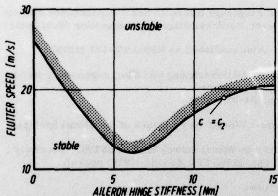
Fig. 22: Flutter speed of the "linearized" wing aileron wind tunnel model as function of changes of the linear hinge stiffness
