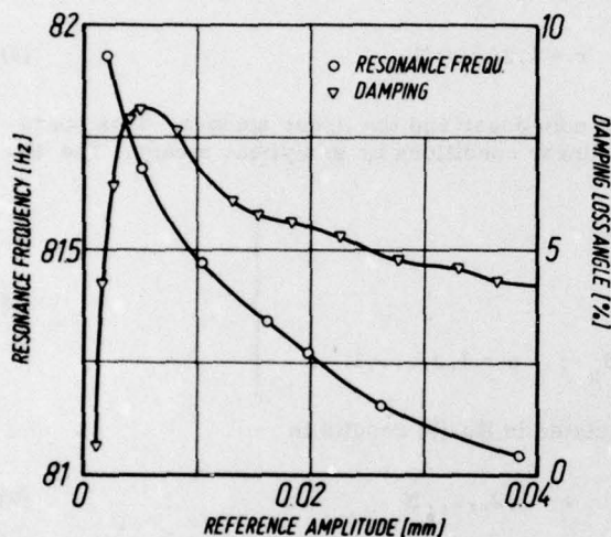
Fig. 9: Structural damping and resonance frequency of a typical F104G normal mode versus reference amplitude
