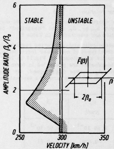
Fig. 13: Effect of hysteresis on the flutter stability of a wing aileron section
