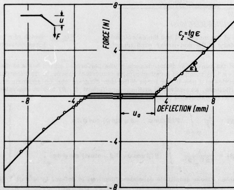
Fig. 18: Non-linear force deflection diagram of the aileron of the wind tunnel test model
