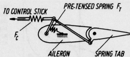
Fig. 5: Sketch of a spring tab mechanism
