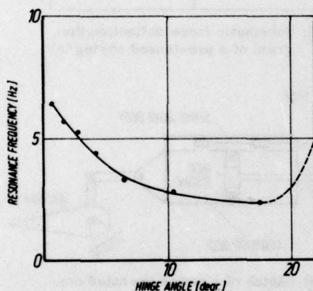
Fig. 3: Resonance frequency of the anti-symmetrical aileron vibration versus hinge angle
