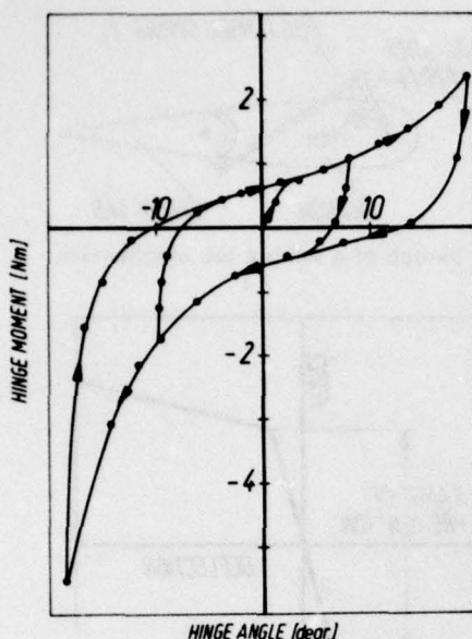
Fig. 2: Aileron hinge moment of a glider versus hinge angle, anti-symmetrical loading
