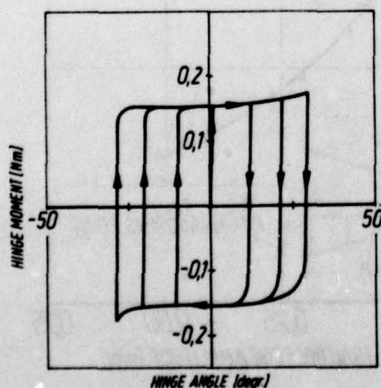
Fig. 4: Rudder hinge moment of a glider versus hinge angle
