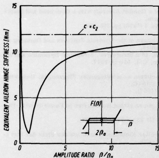
Fig. 21: Variation of the equivalent aileron hinge stiffness of the wind tunnel model versus hinge angle ratio \beta/\beta_a
