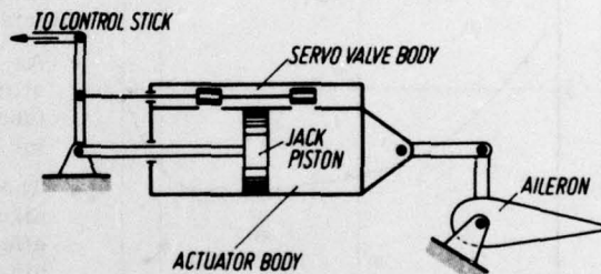
Fig. 7: Sketch of a power operated control surface
