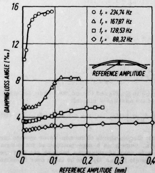
Fig. 10: Structural damping of a fiber reinforced composite box spar as function of vibration amplitude and frequency
