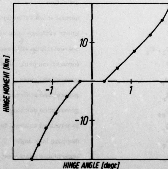
Fig. 1: Aileron hinge moment of a glider versus hinge angle, symmetrical loading
