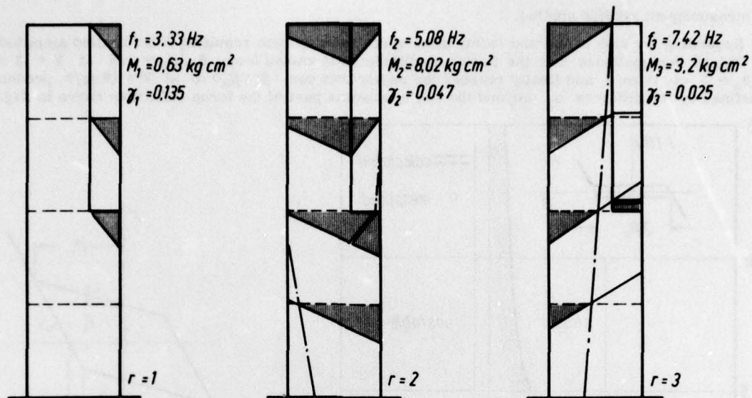
Fig. 17: Normal mode characteristics of a wing aileron wind tunnel test model
