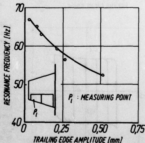
Fig. 8: Resonance frequency of the F 104G aileron vibration versus trailing edge amplitude
