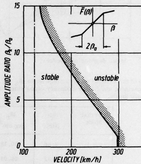
Fig. 14: Effect of a softening spring tab type stiffness on the flutter stability of a wing aileron section
