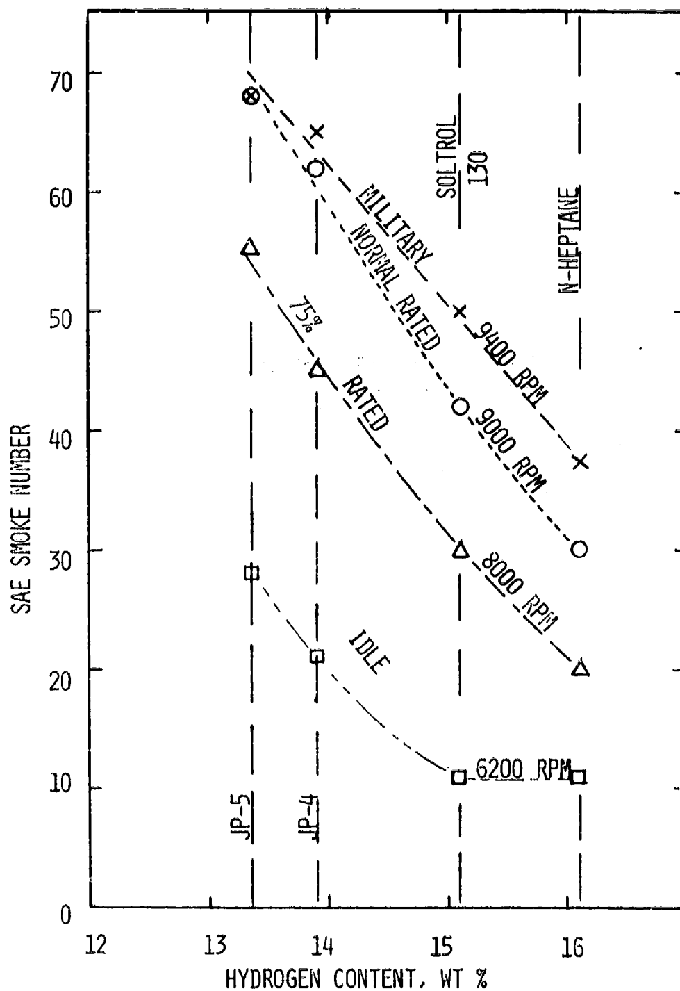
Figure E-2. Fuel Type Effects on Smoke Emitted by J57-P8
