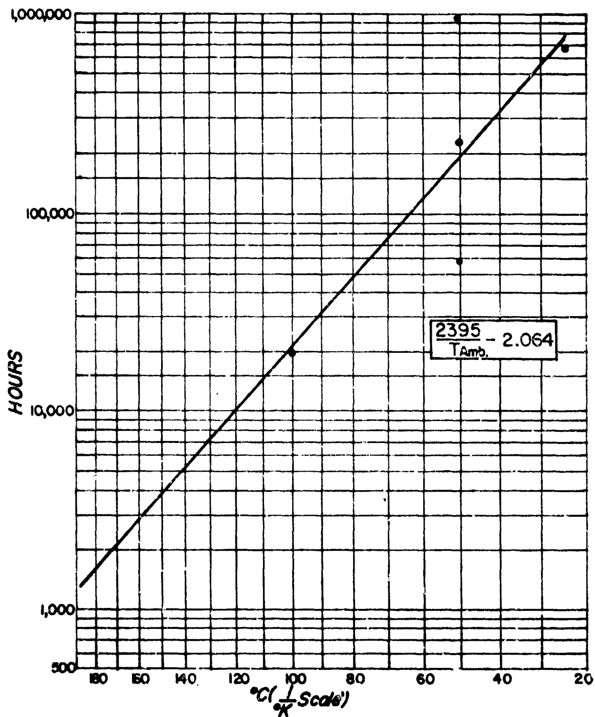
Figure 6 Winding Life Versus Ambient Temperature
