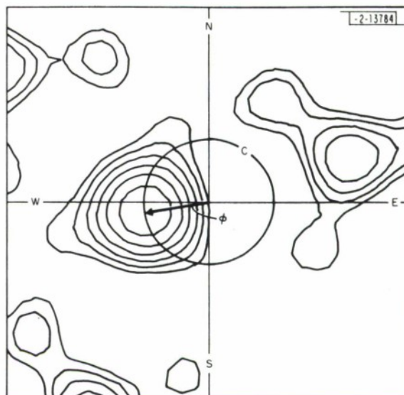
Fig. III-30. Conventional wavenumber spectrum of UH-1 at 8 km. True azimuth is \phi .
