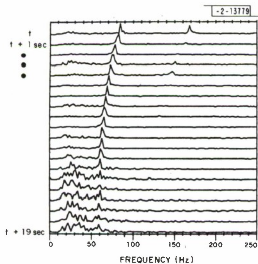
Fig. III-25. Power spectra on a linear scale for a series of 1-sec (1 sec = 110 m position change) time intervals. Target is an OV-1D inbound at an initial range of 1 km.
