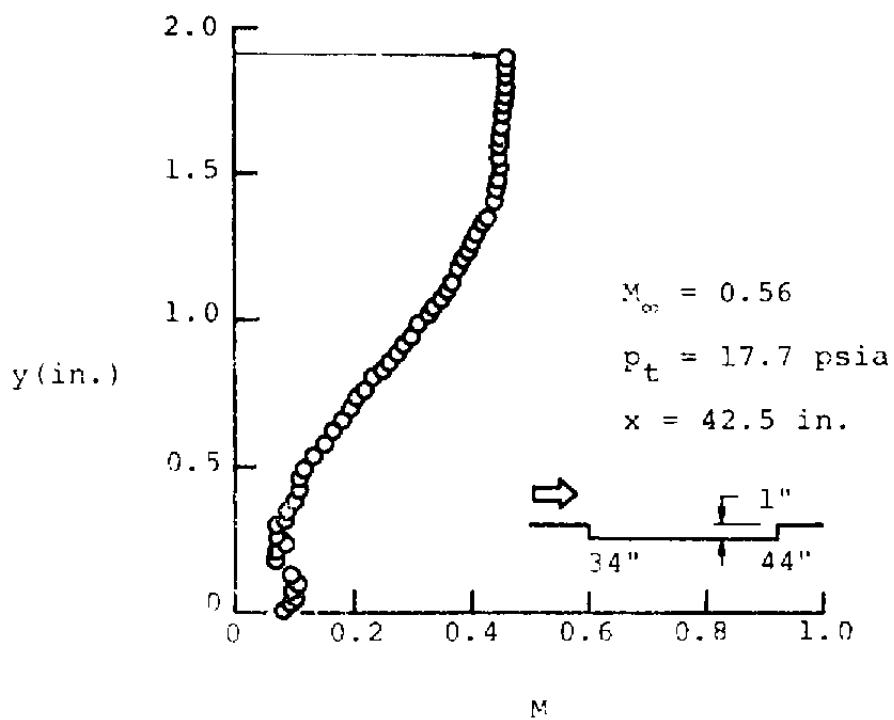
Figure 61. Velocity profile on the 11-inch shallow-cavity model.
