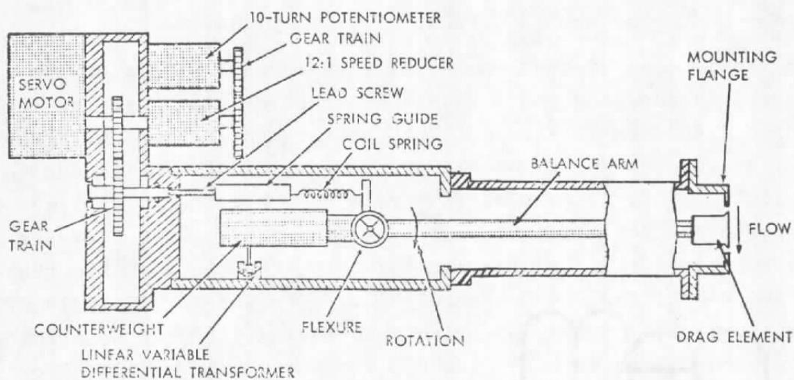
Figure 10. Balance schematic.
