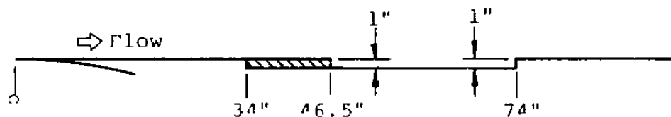
c. 27.5-inch long shallow-cavity model
