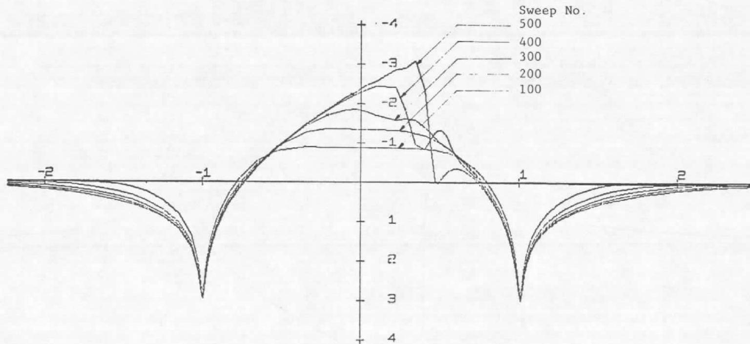
Figure 94. Development of C_p distribution.
