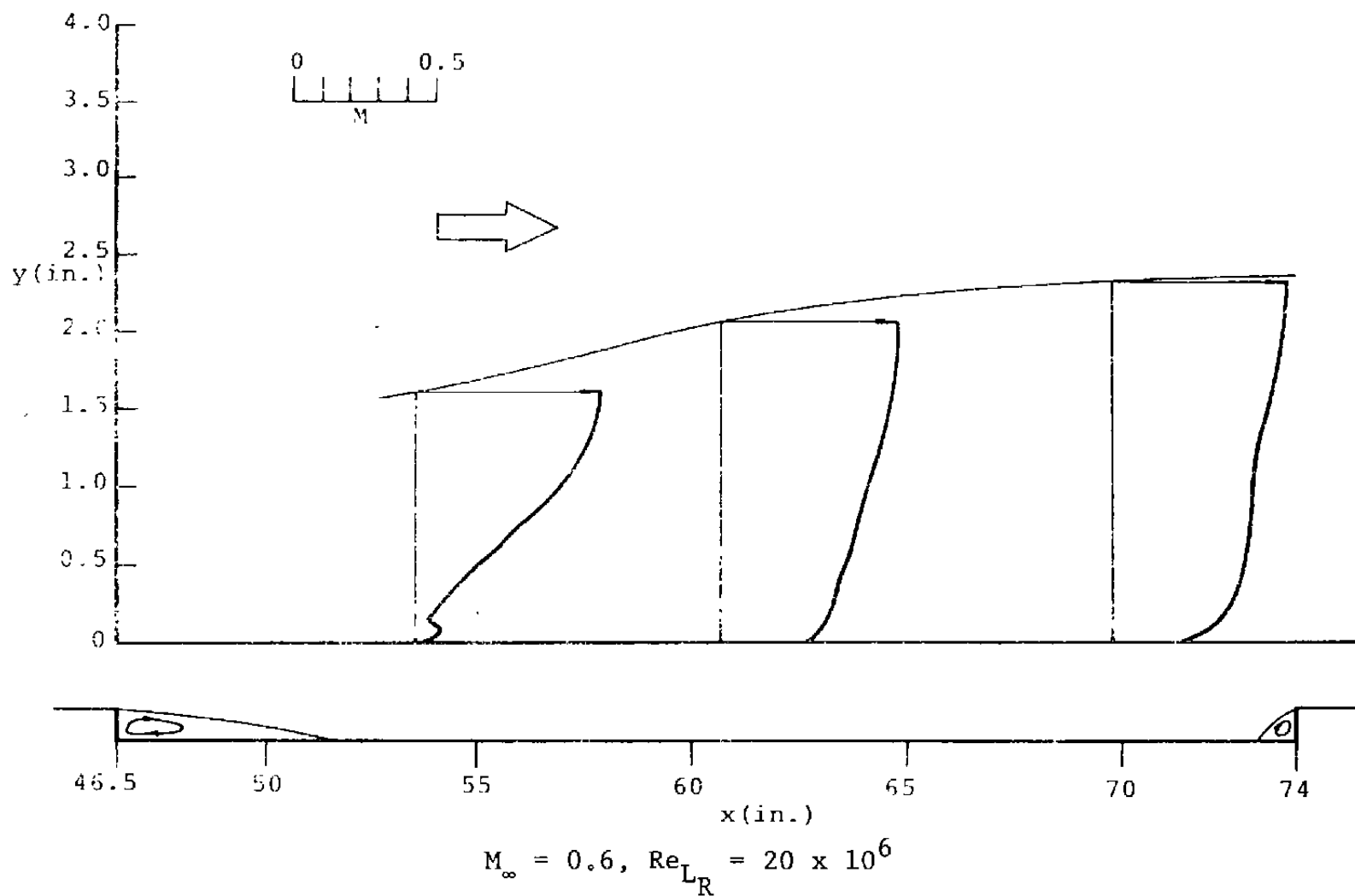
Figure 65. Flow variation along the 27.5-inch cavity model.
