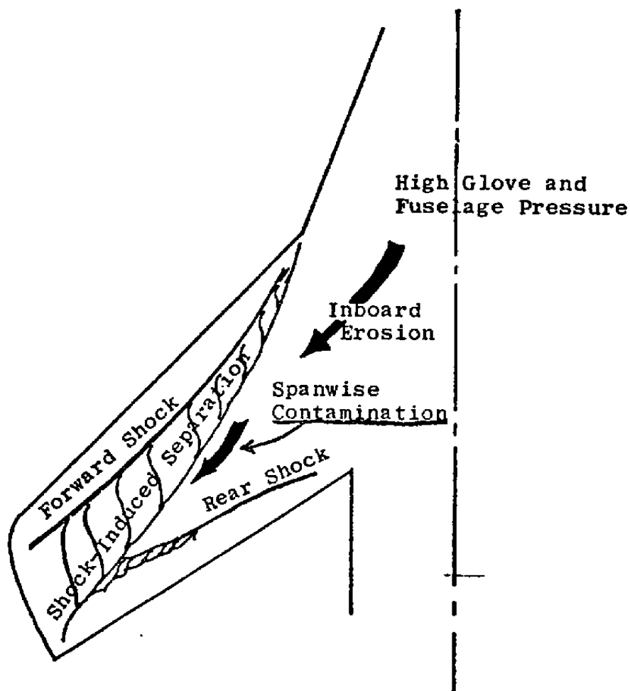
Figure 2. Shock and separation pattern at 45^\circ sweep, M_\infty = 0.95 and \alpha = 9^\circ (Ref. 3).
