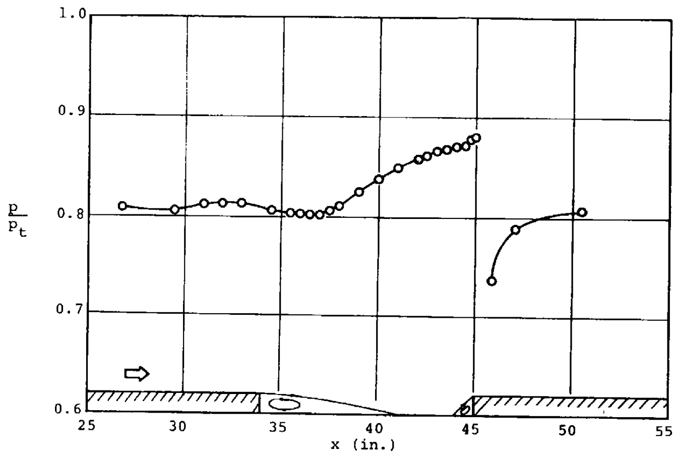
Figure 11. Surface pressure distribution along 11-inch cavity.
