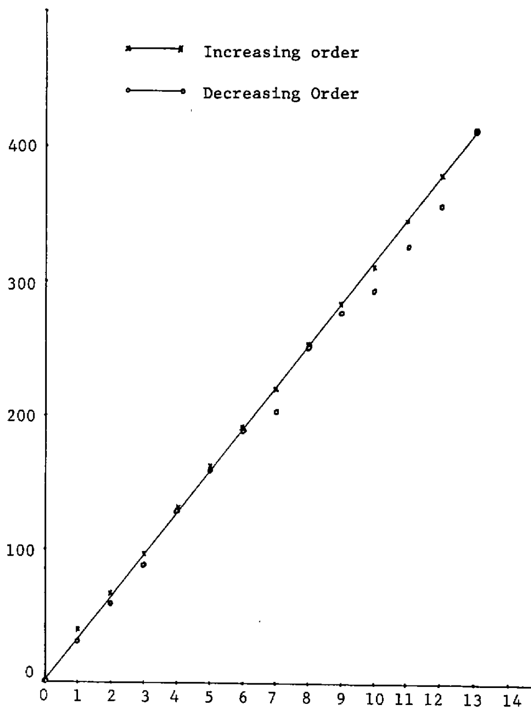
Figure 91a. Calibration curve of skin friction meter mounted in UTSI Transonic Wind Tunnel.
