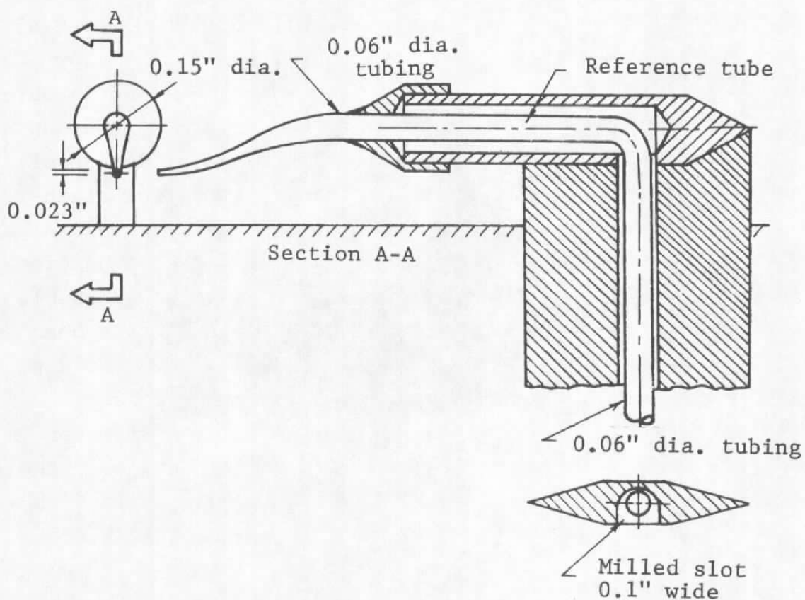
a. Cross-sectional view (schematic)
