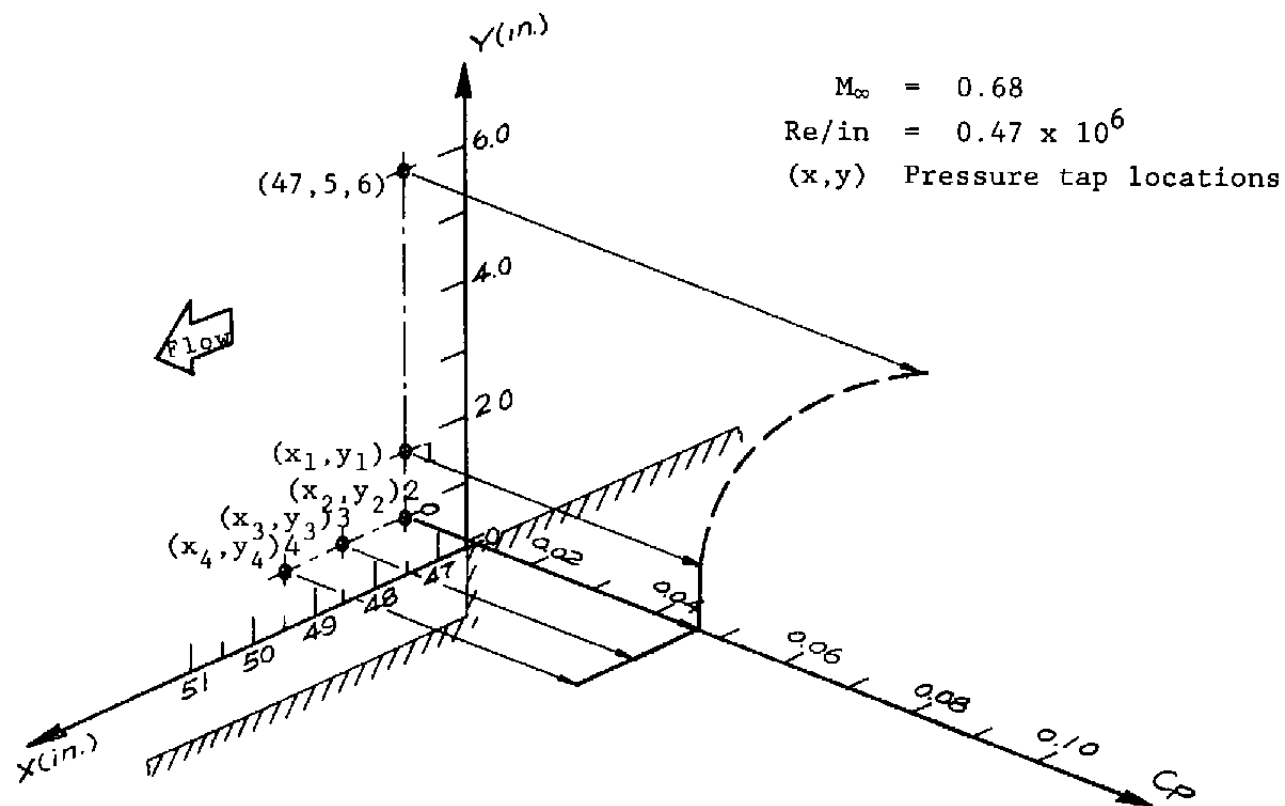
Figure 18. Static pressure distribution on the side wall near the rearward-facing step region.
