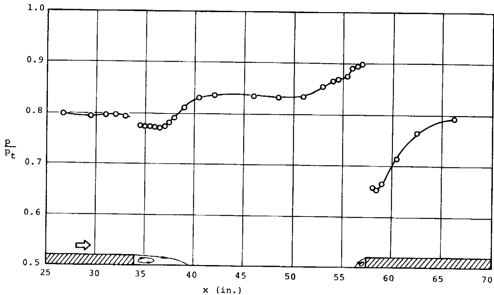
Figure 13. Surface pressure distribution along 23.5-inch cavity.
