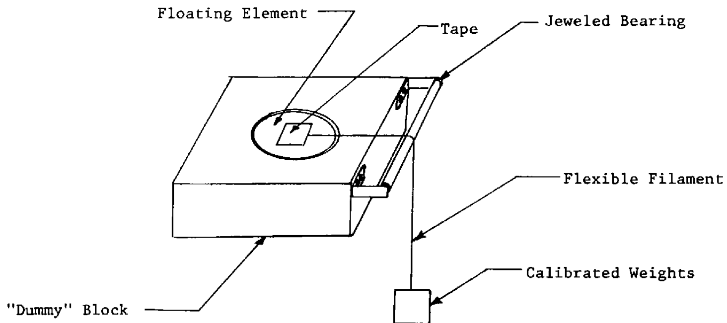
Figure 90. Calibration technique.
