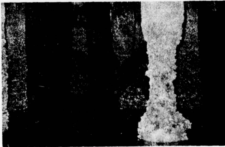
Pile in foreground with classic Limnoria 'hourglassing', two other piles completely destroyed.
