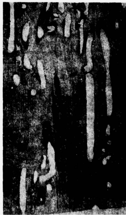
Longitudinal Section of Same Pile showing the eccentricity of the voids and extensive loss of cross-section.
