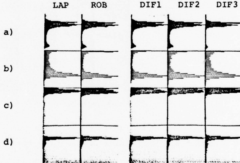
Figure 5. Histograms for the four images in which points having low edge values are given higher weights.
