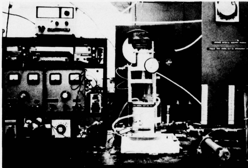
Figure 19. Overview of the freeze-thaw consolidation setup
