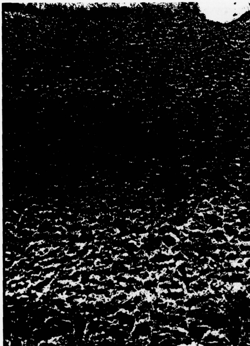
Figure 35. Magnification of 7× of a vertical thin section of the Toledo Penn 7 material after freezing
