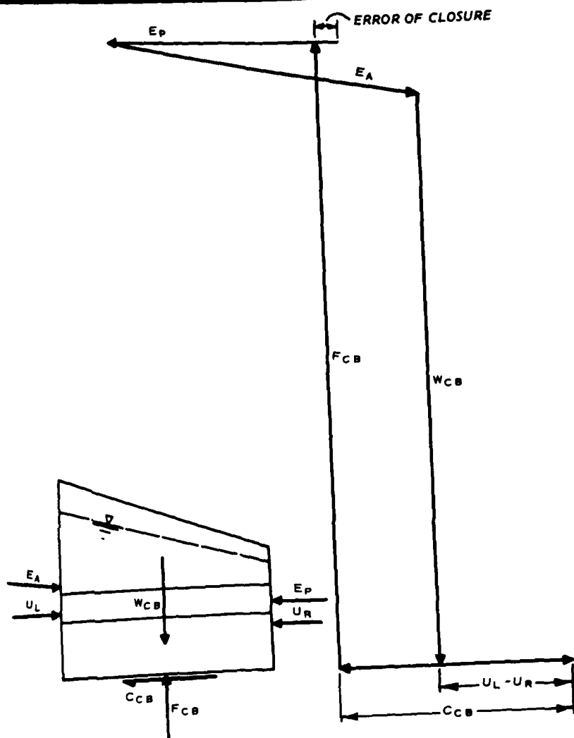
FORCES ON CENTRAL BLOCK AND FORCE POLYGON, FS = 1.27
