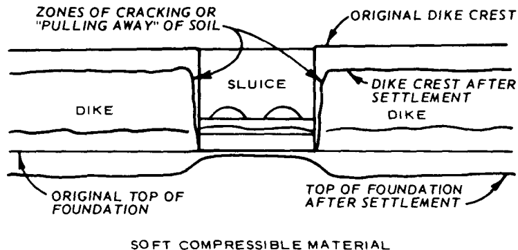
Figure 26. Cracking at dike-structure junction caused by differential settlement caused by dike load on foundation being much greater than sluice load
