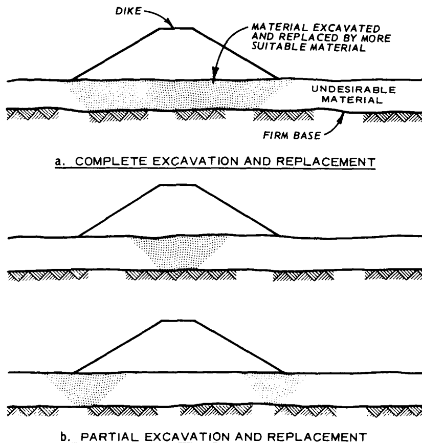
Figure 37. Typical use of excavation and replacement method to improve stability
