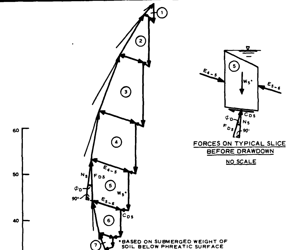
FORCE POLYGON FOR ARC SHOWN AT RIGHT, FS = 1.78 BEFORE DRAWDOWN
