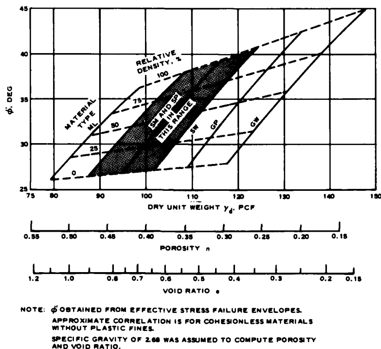
Figure 6. Angle of internal friction versus density for coarse-grained soils (after Reference 17)
