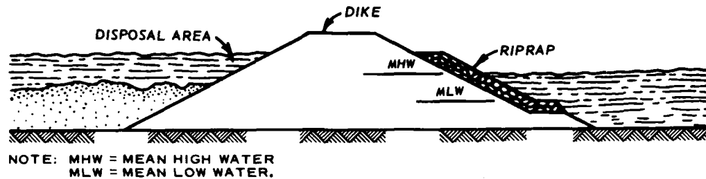
Figure 48. Cross section of dike with exterior slope protected by riprap (after Reference 26)
