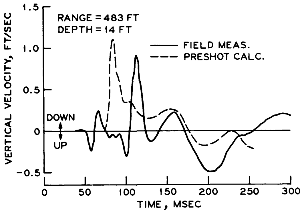
COMPARISON OF MIXED COMPANY CALCULATIONS WITH WES MEASURED FIELD RESPONSE
