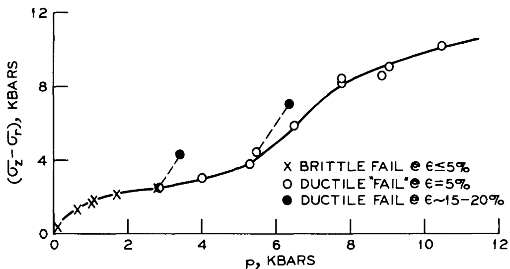
MIXED COMPANY SANDSTONE (LLL AND TT)
