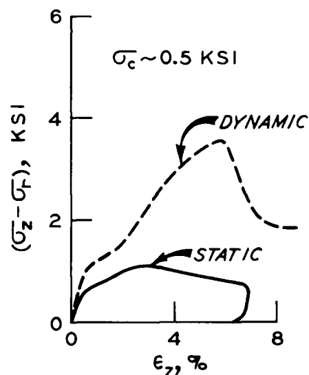
MIDDLE GUST UNWEATHERED SHALE (WES)
