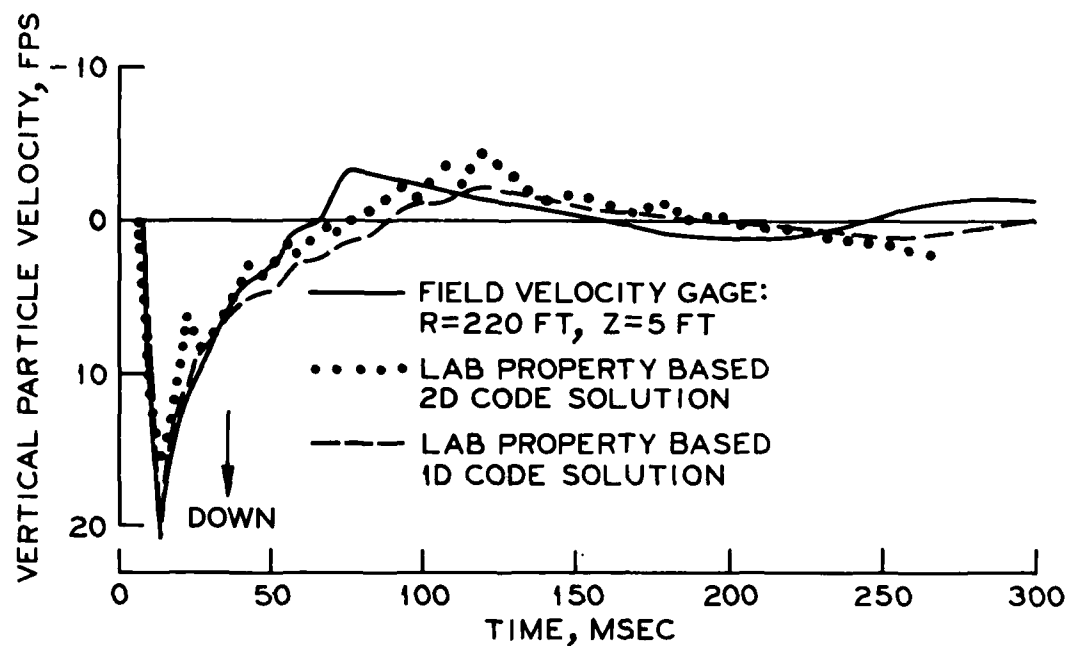
PRAIRIE FLAT AI-ONLY CODE CALCULATIONS-1970
