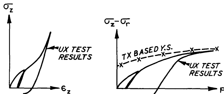
MATERIAL RESPONSE CHARACTERIZATION-1969
