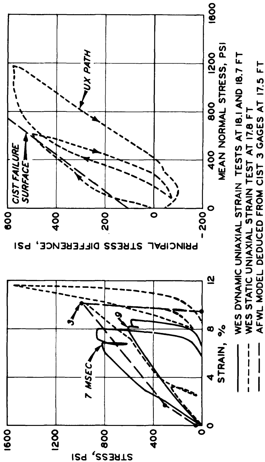
SANDY CLAY FROM MINUTEMAN SITE D-1, KIMBALL, NEB.
