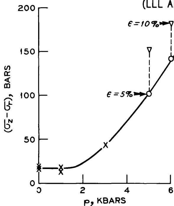
MIDDLE GUST WEATHERED SHALE (LLL)
