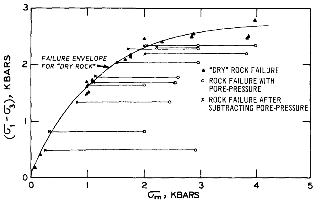
PORE PRESSURE EFFECTS ON MIXED COMPANY SANDSTONE (TERRA TEK)
