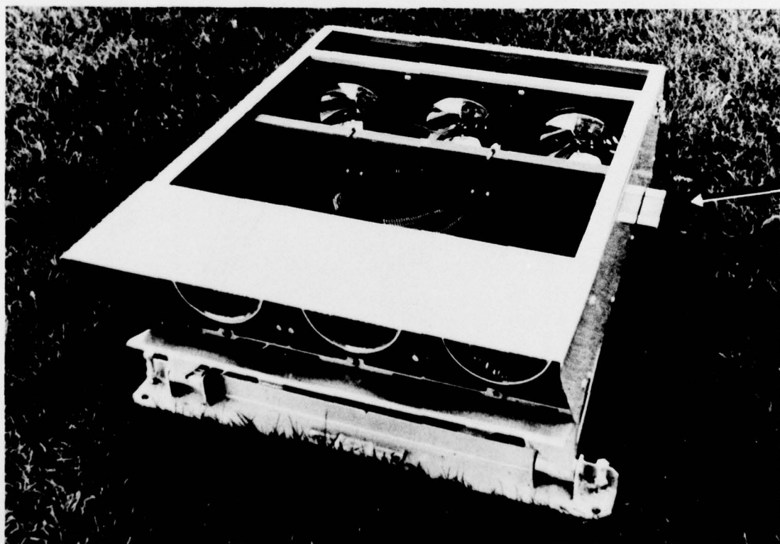
Fig.5 PAPI unit
