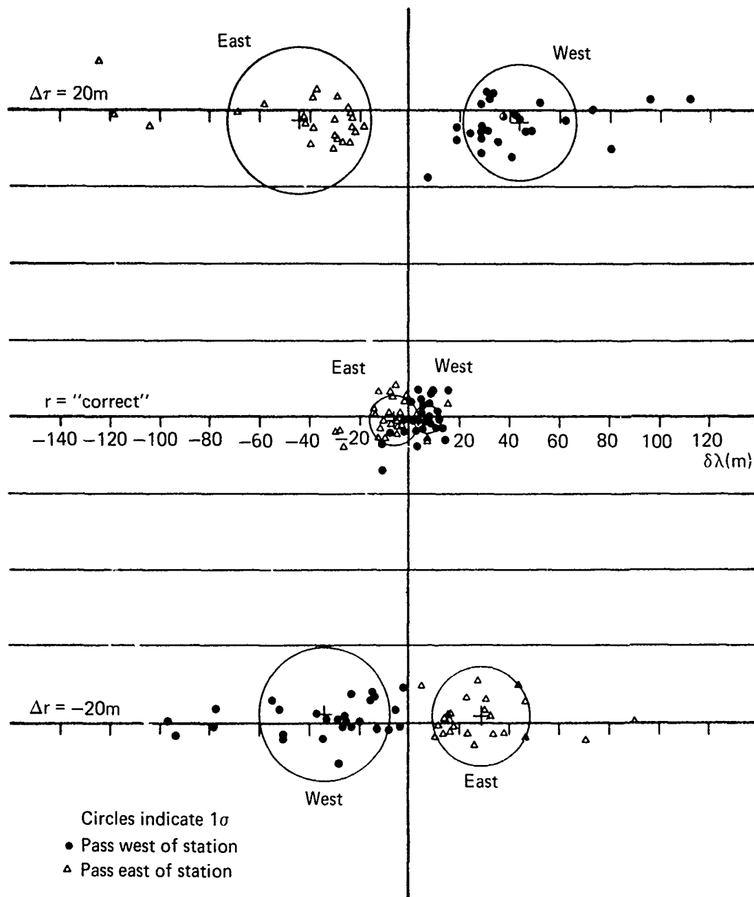
Fig. 11 Determination of the 3-Dimensional Position (all satellites, days 40-43, 1974).
