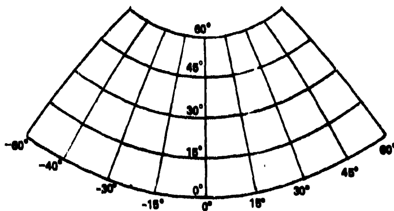
Figure 6.5.2. Transverse polyconic projection
