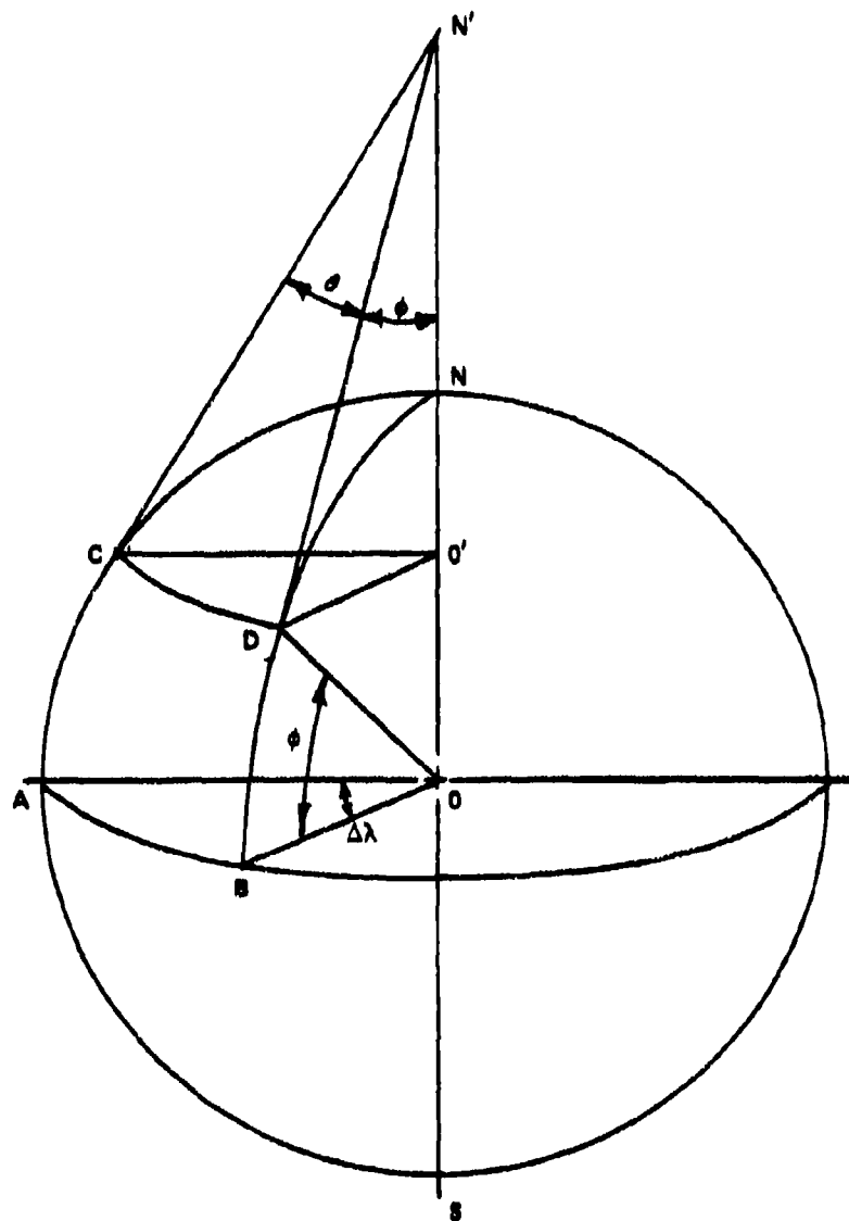
Figure 2.9.1. Geometry for angular convergences of the meridians
