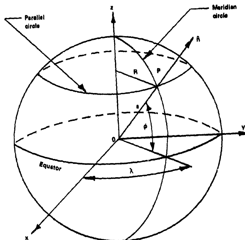
Figure 3.B.1. Geometry of the sphere
