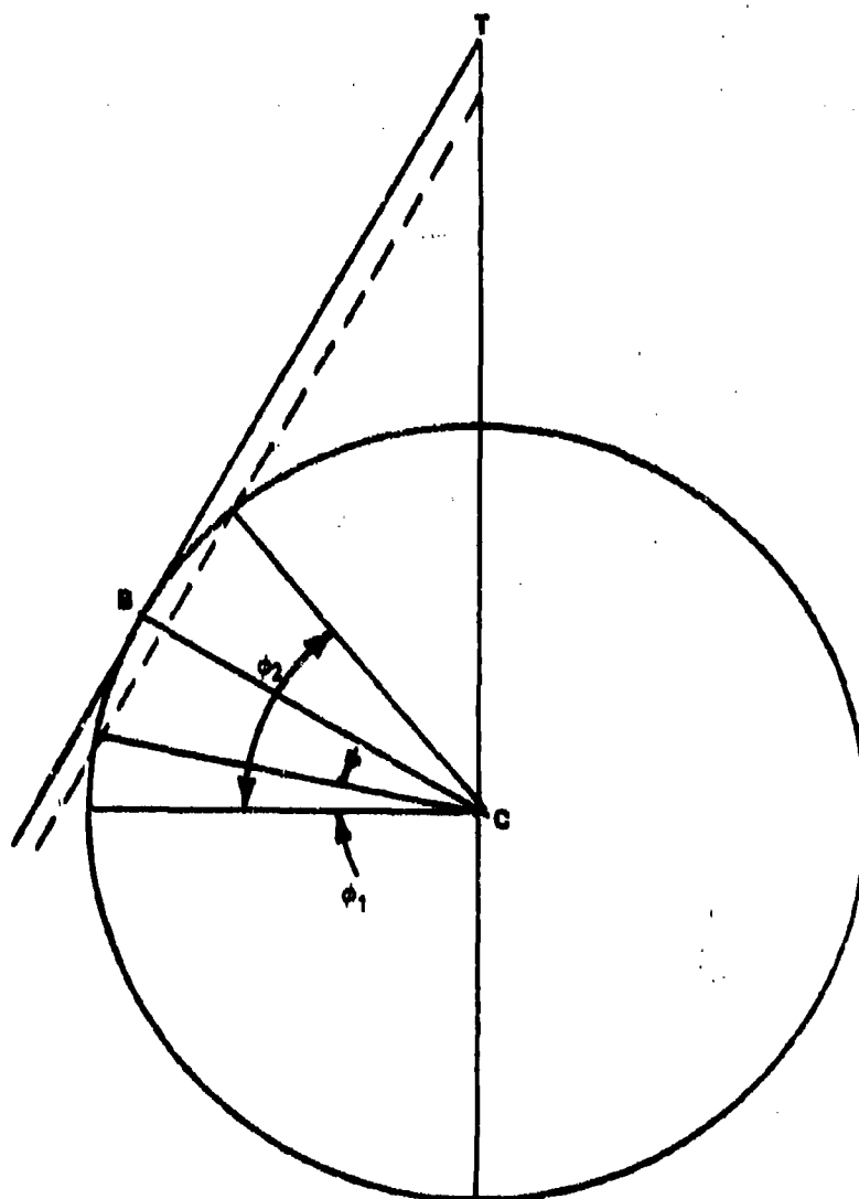
Figure 6.12.1. Geometry for the Murdosch projection
