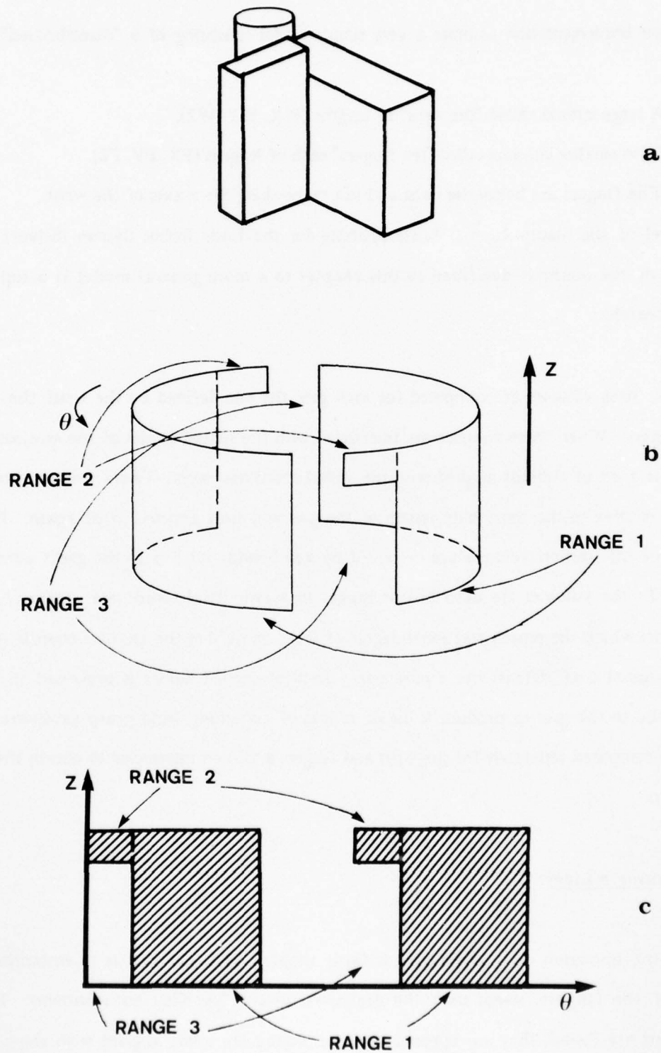
Figure 4.6 - PGSET[l] example. (a) is the object to be grasped, we consider grasping the cylinder. (b) shows the surface of legal positions for the fingers. (c) is a planar representation of (b).
