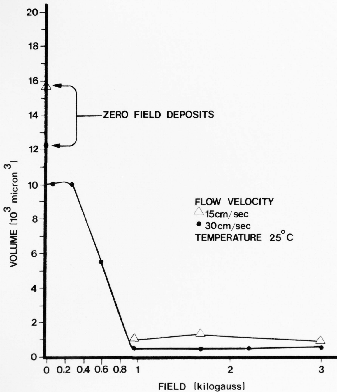
ENTRY DEPOSIT VOLUME VS. MAGNETIC FIELD MOBIL II SEEDS
