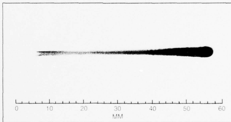
FERROGRAM
