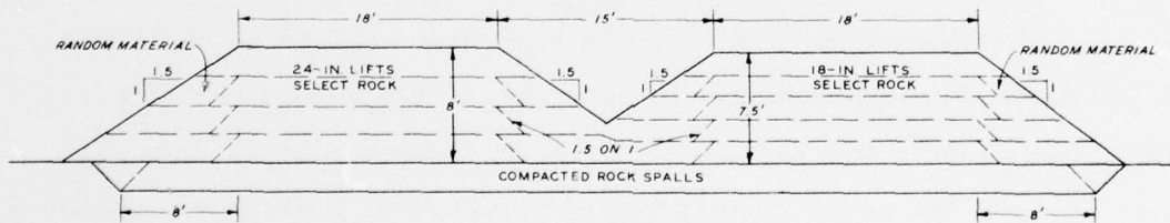
SECTION C-C
