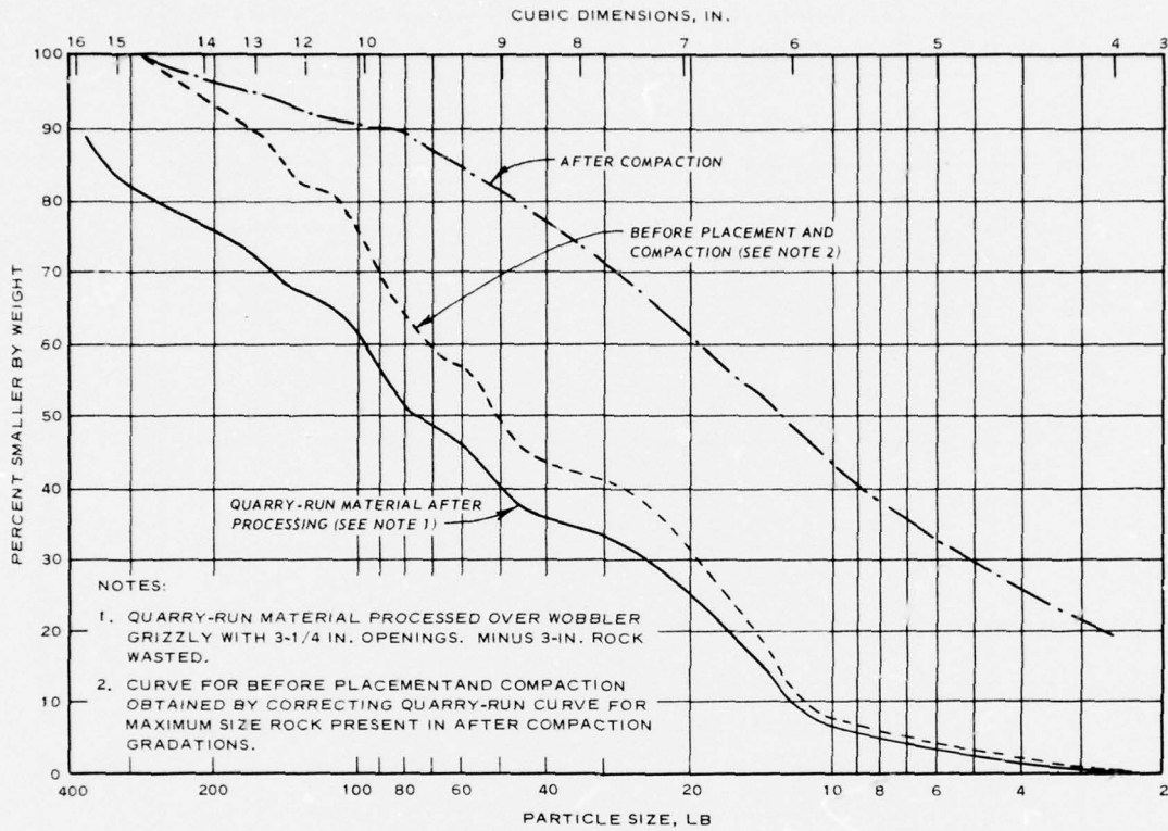
Fig. 58. Before- and after-compaction gradation curves, panel 6, Gilham test fill
