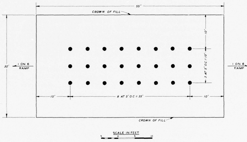
Fig. 32. Grid for settlement readings, New Melones test fill
