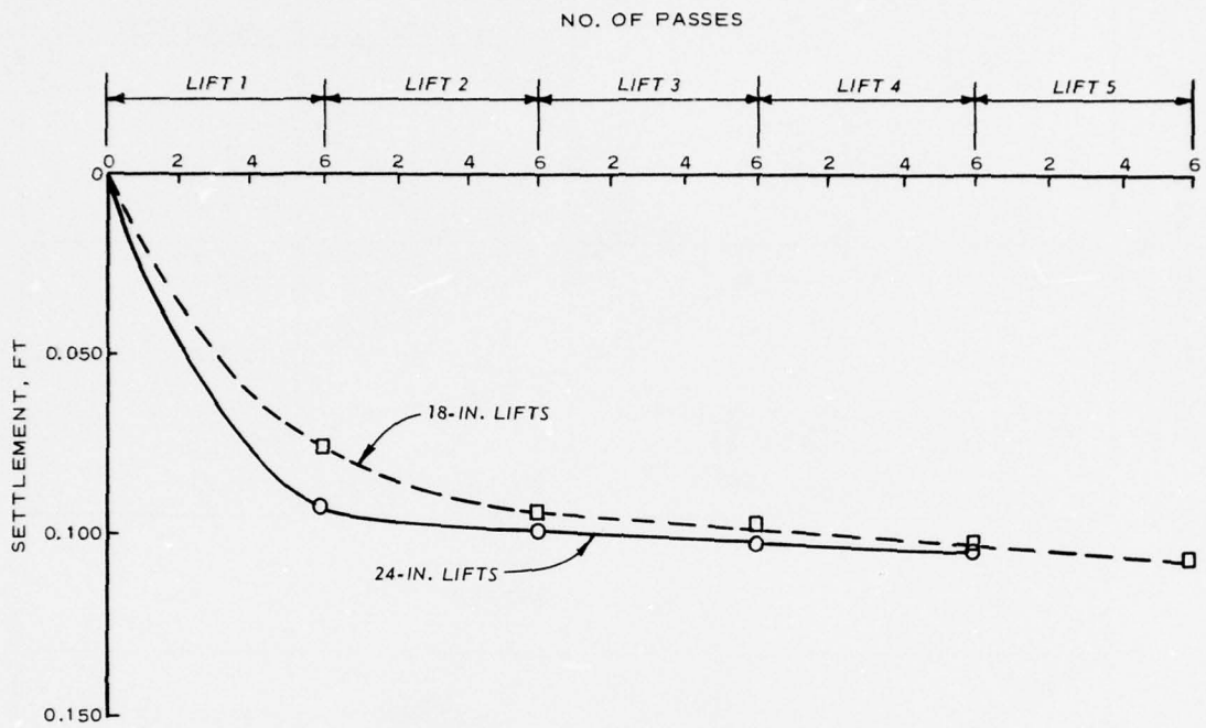
Fig. 24. Foundation settlement, Gathright test fill
