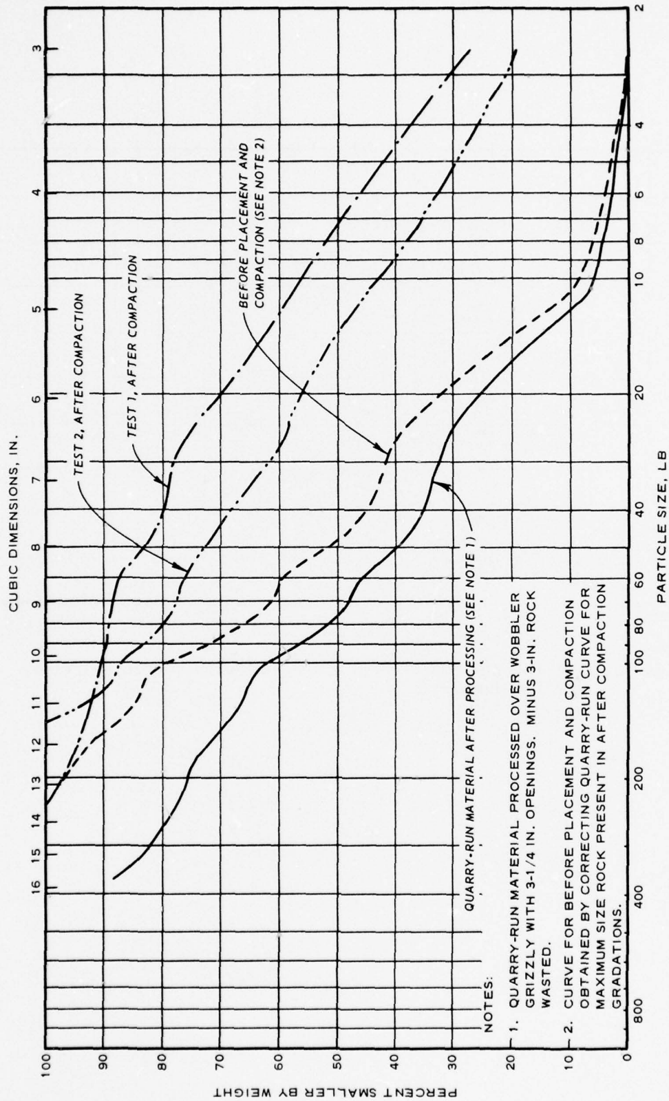
Fig. 57. Before- and after-compaction gradation curves, panel 5, Gilliam test fill
