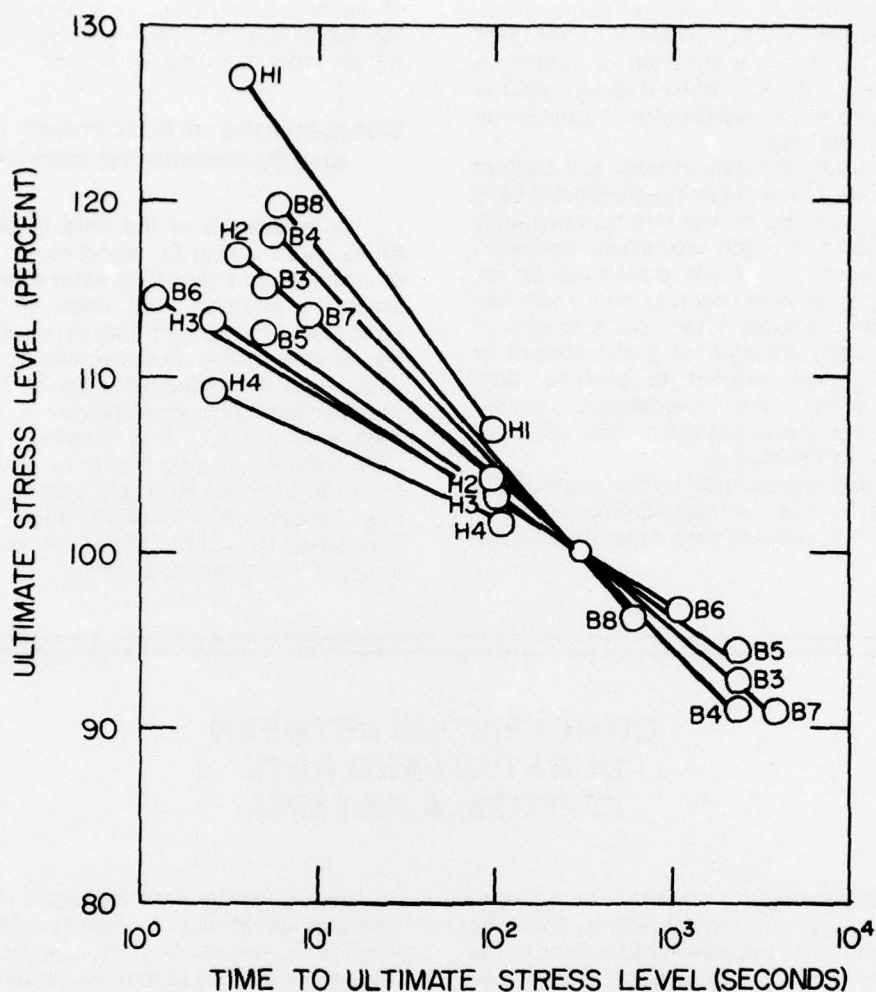
Figure 8.--Typical loading rate relationships for wood-based materials--ultimate load versus time to ultimate load. (Numbers refer to itemized data in table 5.)
