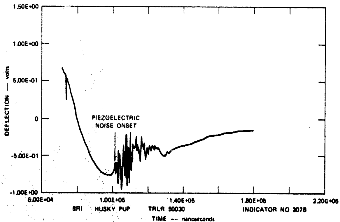
FIGURE 16 HUSKY PUP TIME-OF-ARRIVAL SIGNAL
