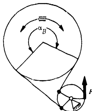
Figure 2-22. Inline Application External Band Brake
