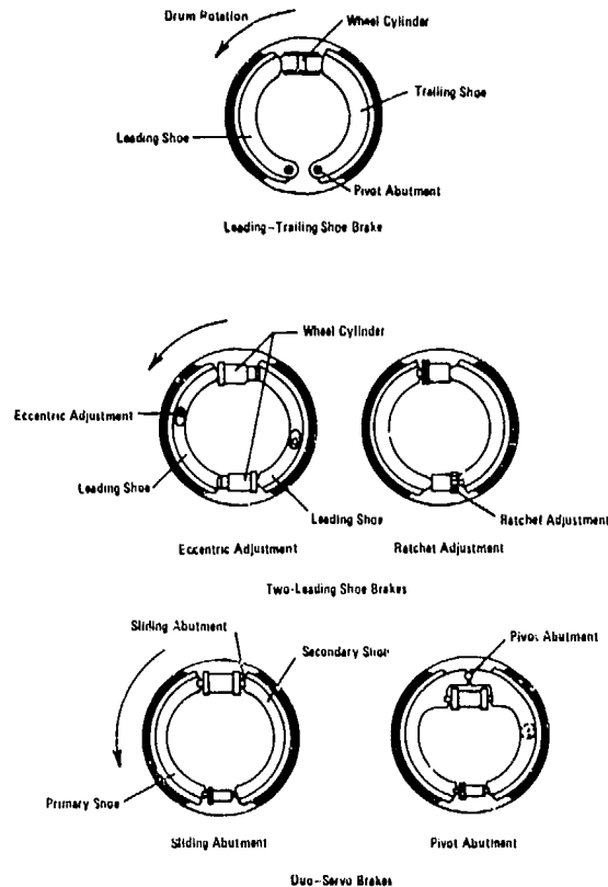
Figure 2-1. Basic Drum Brakes
