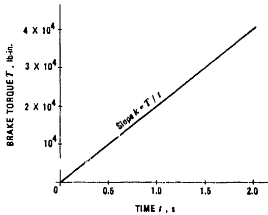
Figure 10-2. Brake Torque Rate — Induced by Driver
