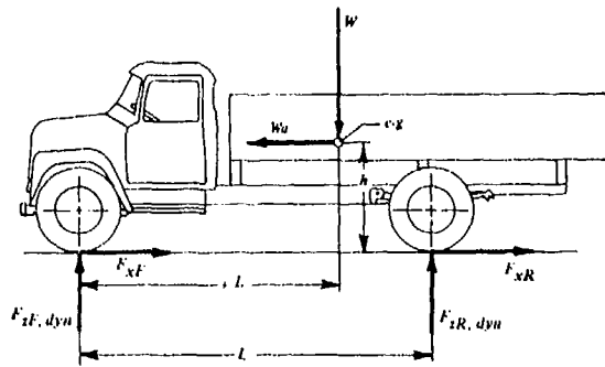
Figure 7-2. Forces Acting on a Decelerating Vehicle
