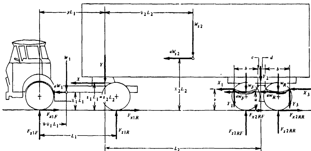
Figure 8-34. Forces Acting on a Tractor-Semitrailer Equipped With Two-Leaf Suspension
