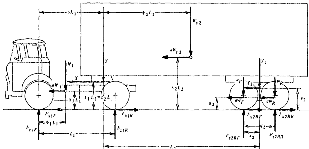
Figure 8-37. Forces Acting on a Tractor-Semitrailer Equipped With Walking Beam Suspension
