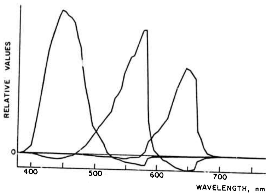
Figure (4-6) Columns of pseudo-inverse operator
