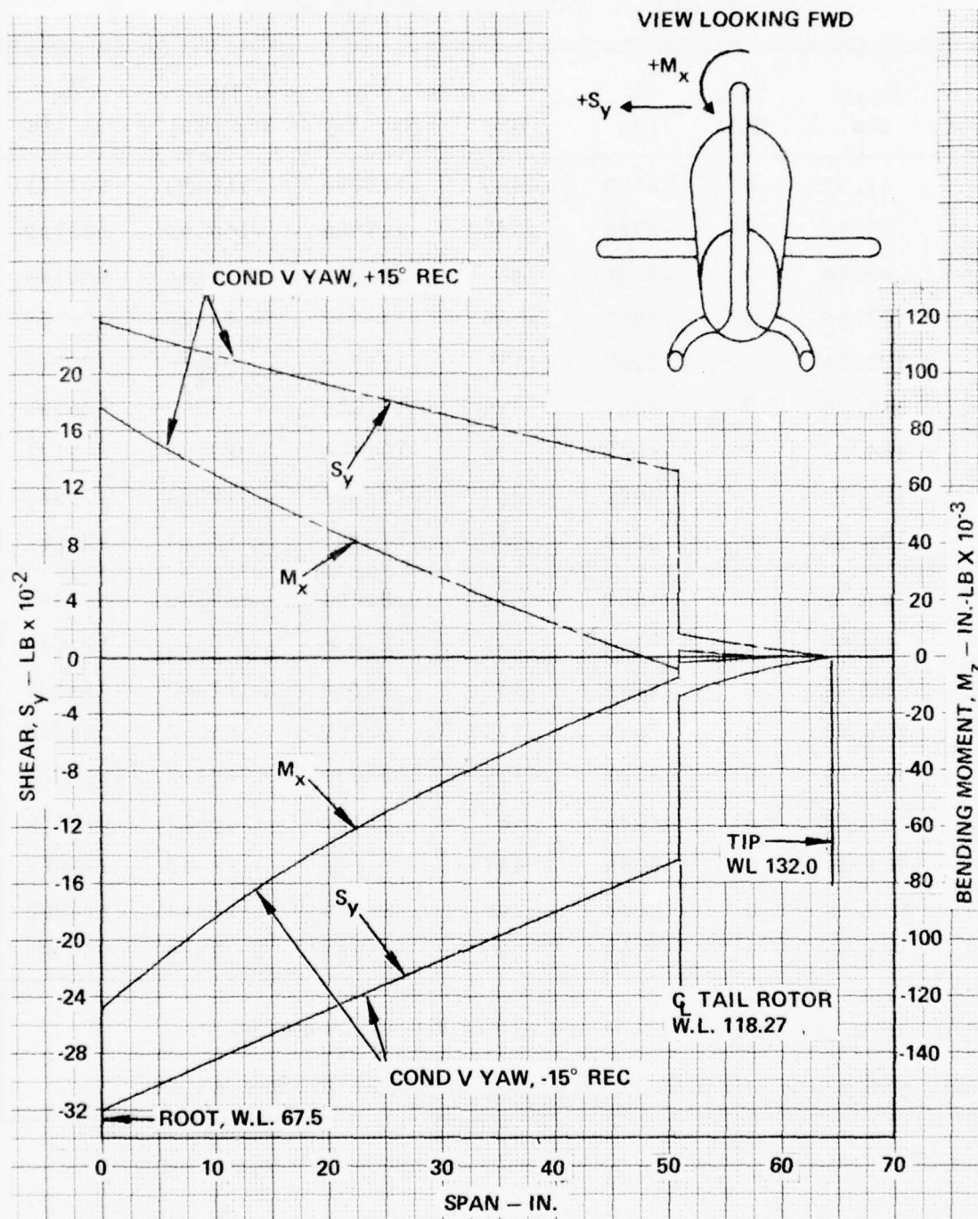
Figure 5. Vertical Fin Spanwise Shear and Bending Moment.
