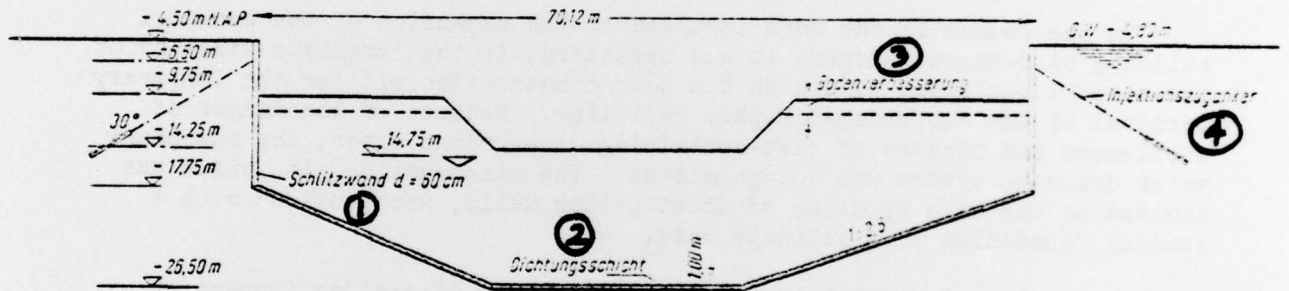
Figure 5. Cross Section, Construction Pit, Computer Center ABN, Amstelveen
