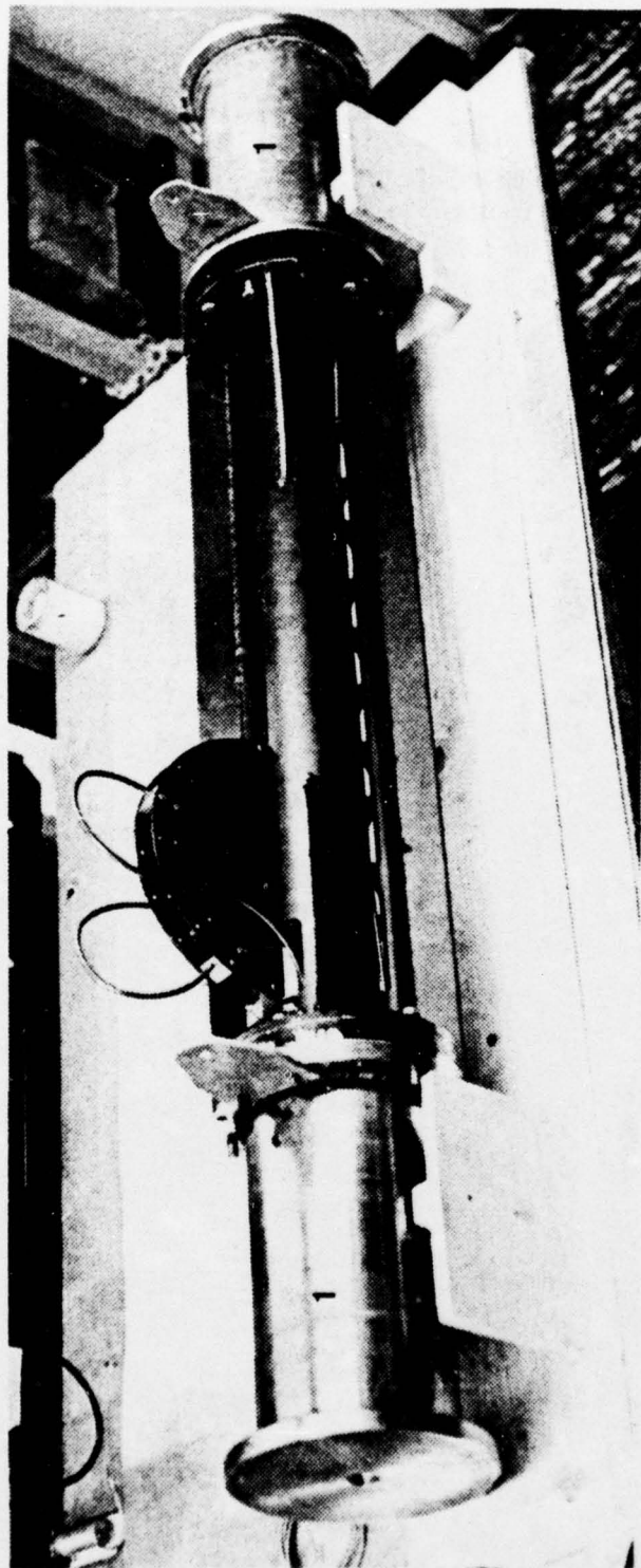
Figure 3. NPS Transmissometer-Nephelometer.
