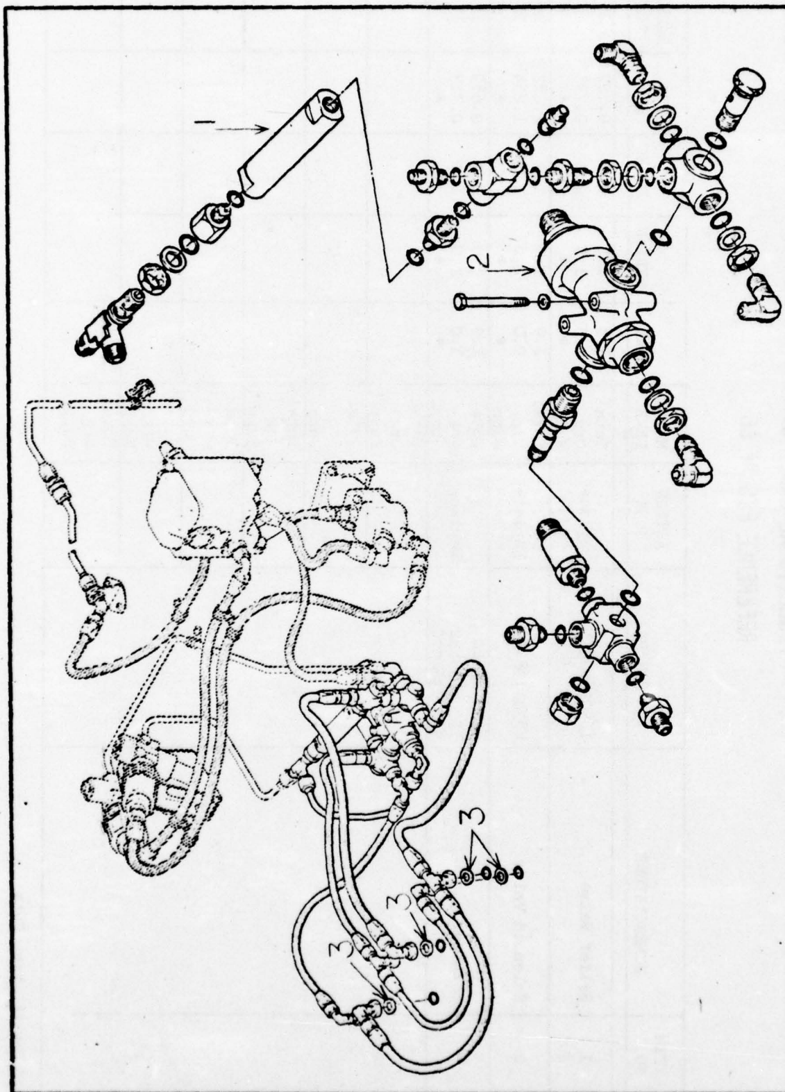
Figure 66 Flight Controls Hydraulic System Installation
