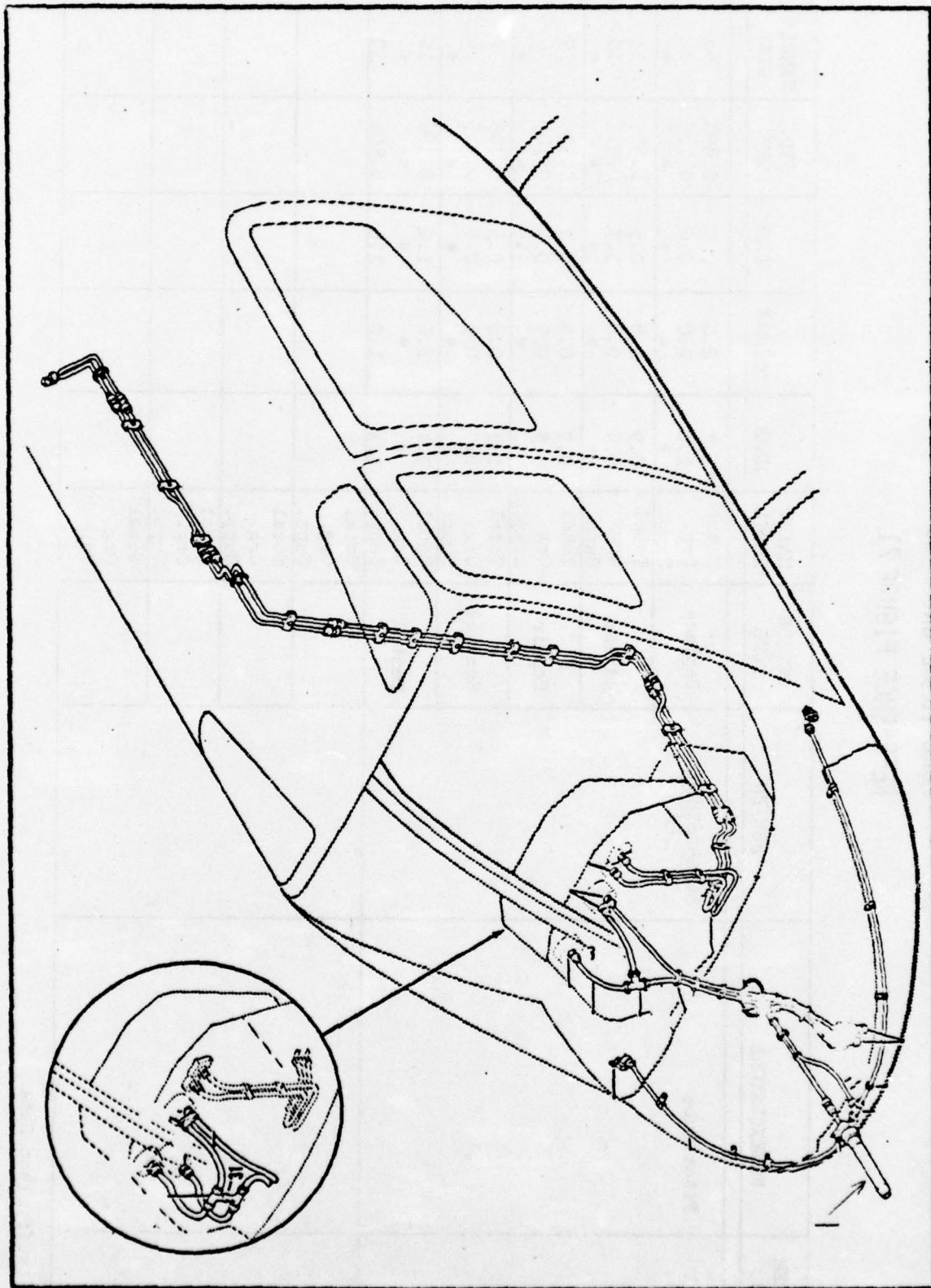
Figure 71 Instrument Piping Installation
