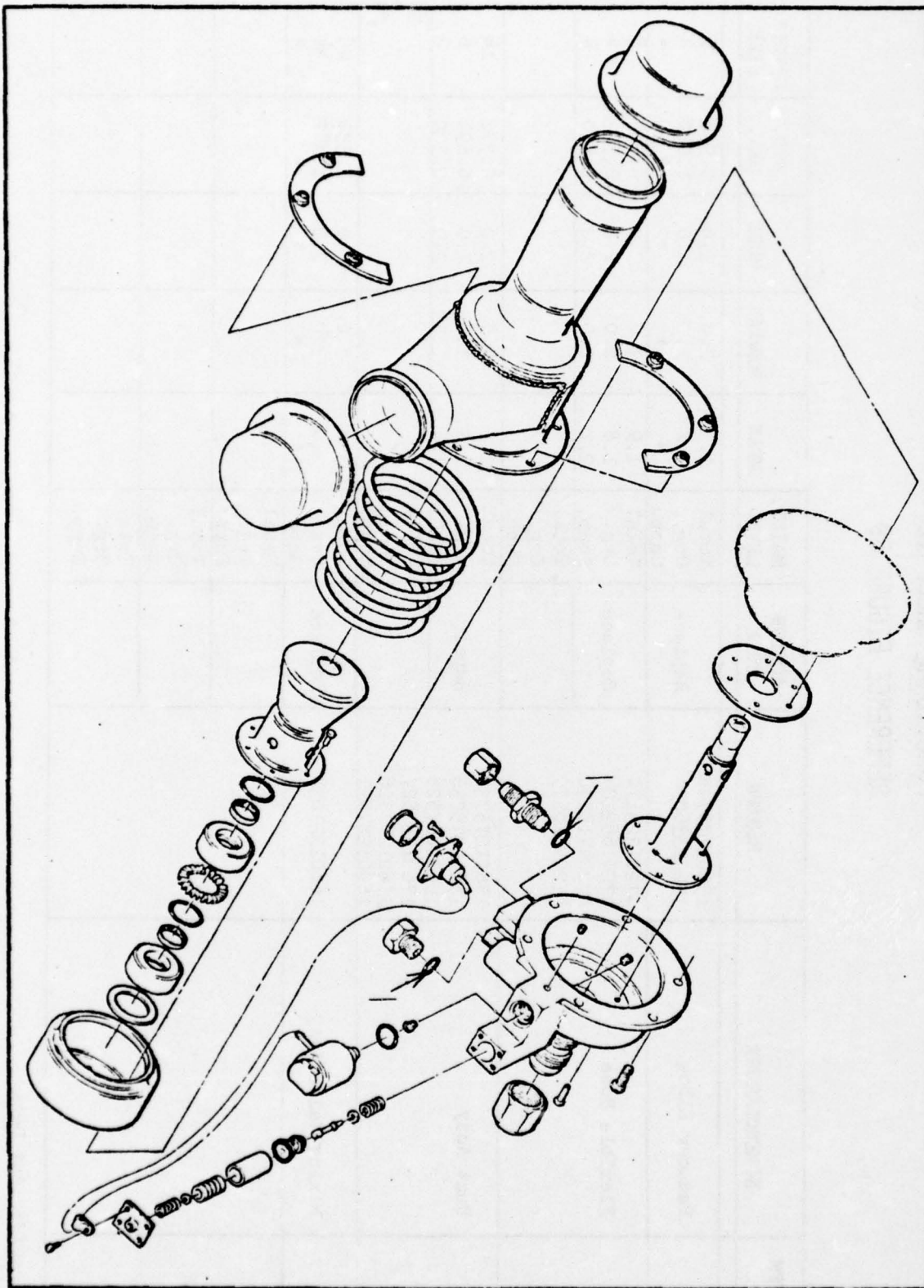
Figure 90 Mixing Valve Assembly
