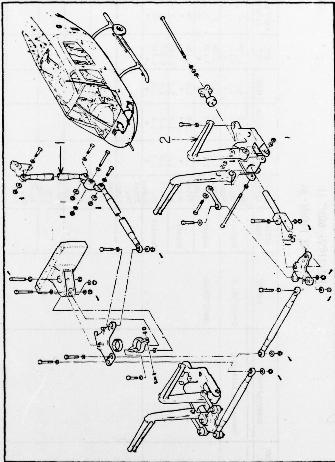
Figure 84 Antitorque System Controls Installation
