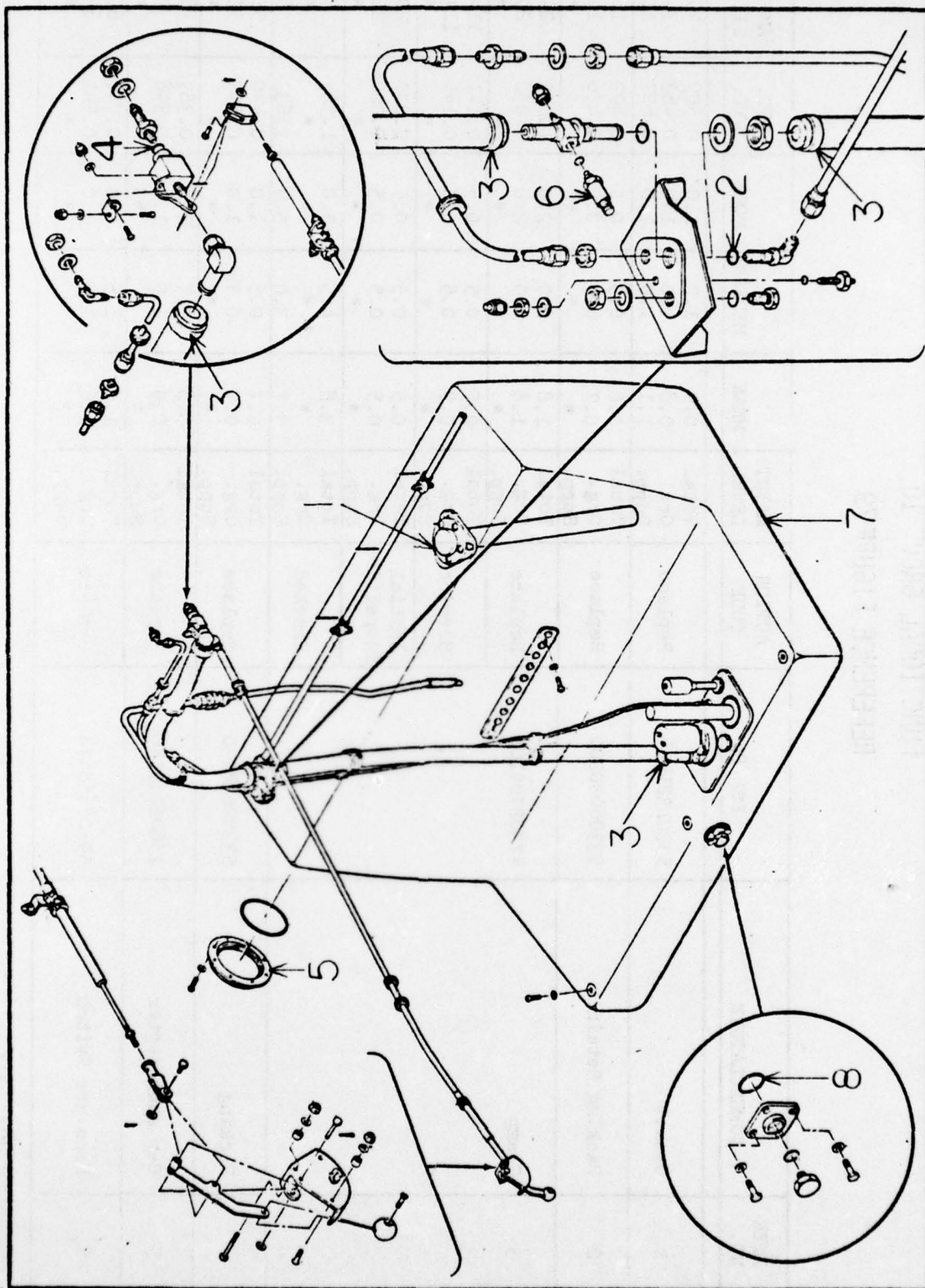
Figure 79 Fuel System Installation
