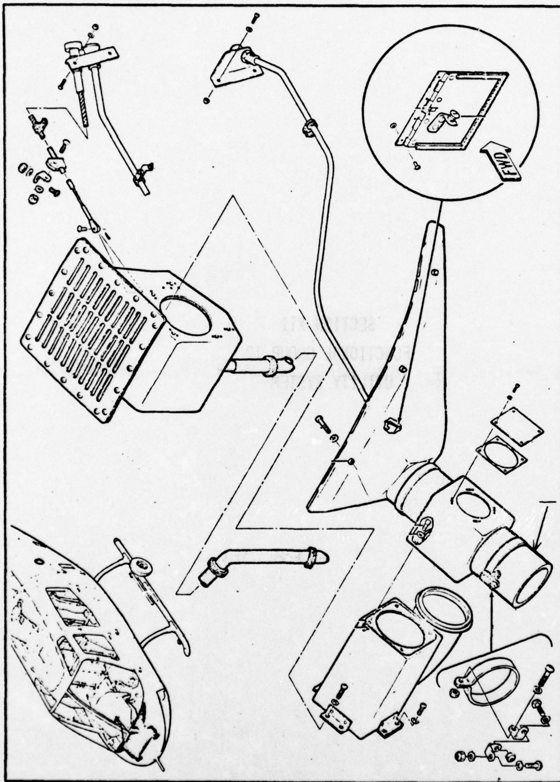
Figure 88 Ram Air and Defogging Ventilation System Installation
