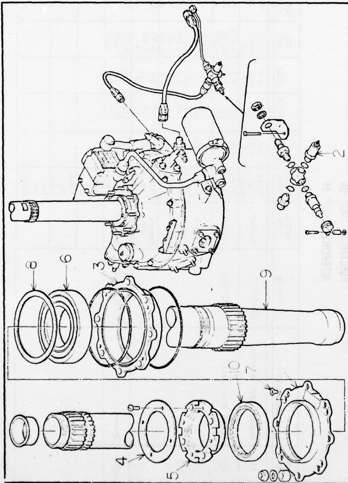
Figure 57 Transmission Installation
