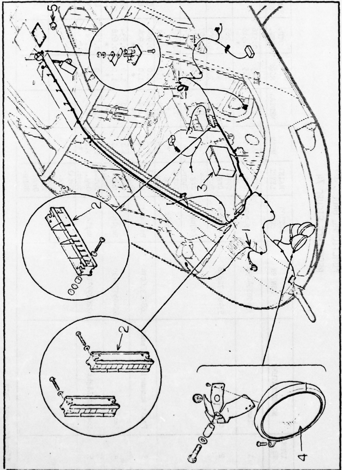
Figure 74 Electrical Installation
