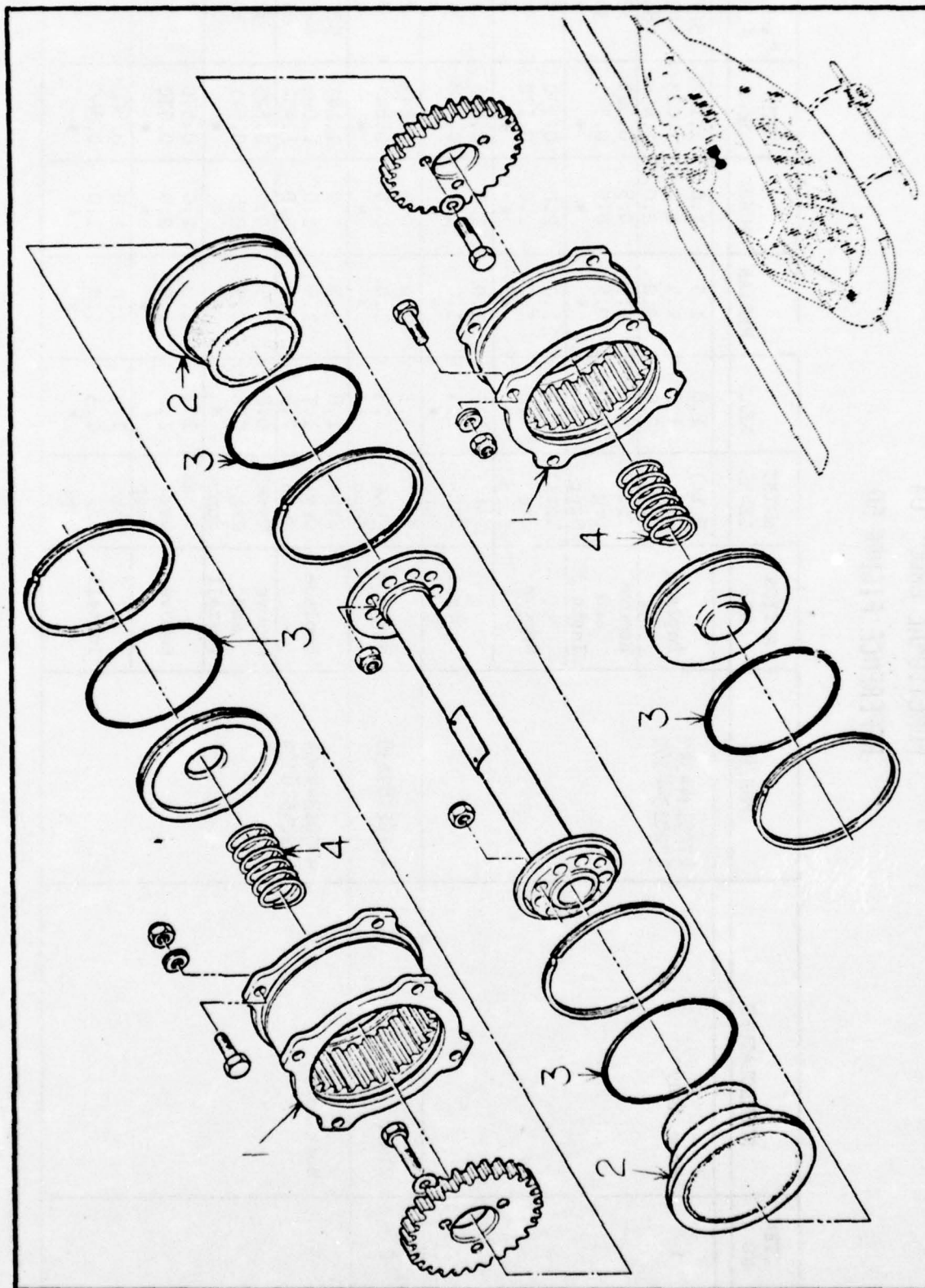
Figure 61 Engine to Transmission Drive Shaft Assembly and Installation
