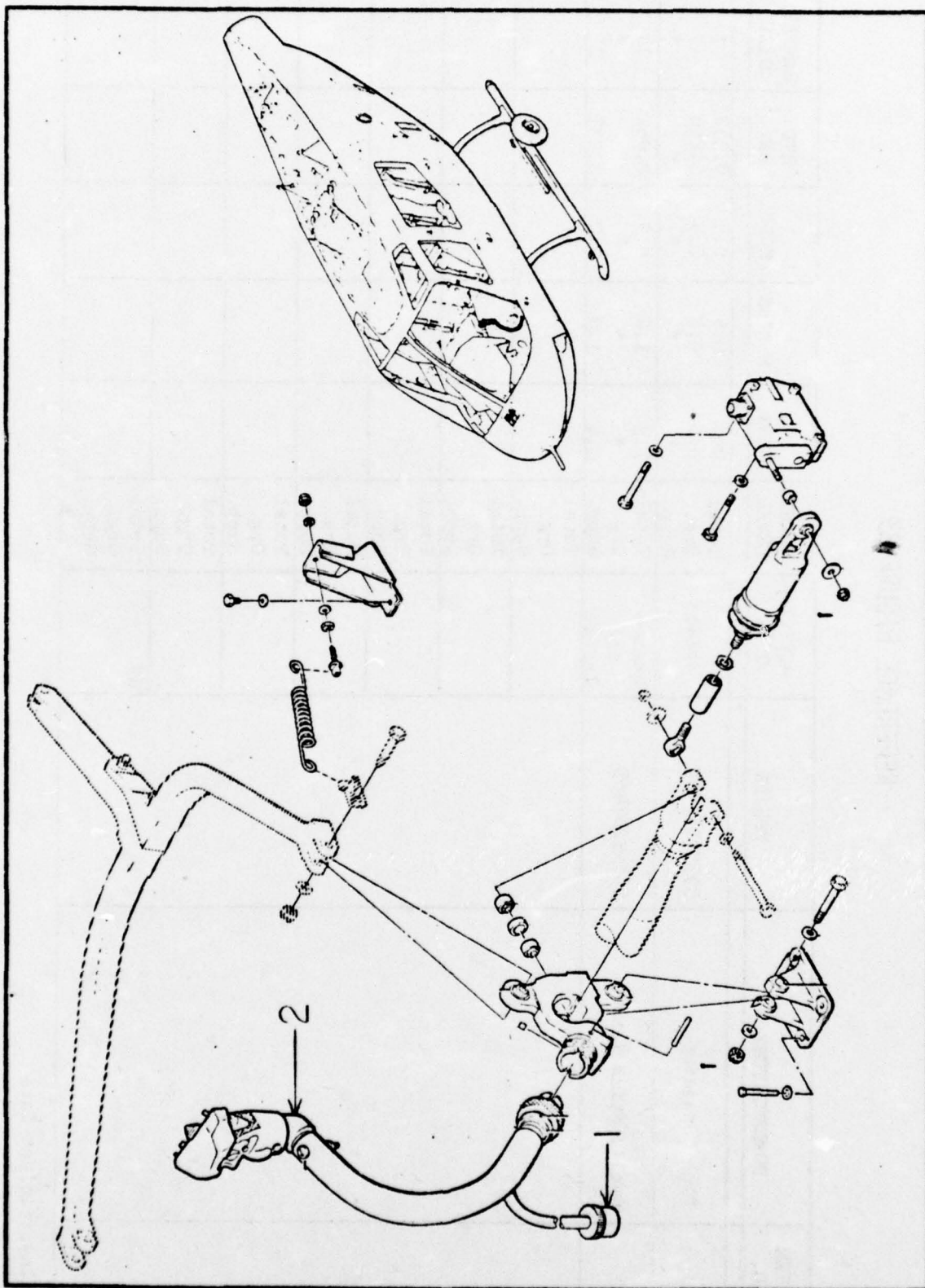
Figure 83 Cyclic Controls Installation
