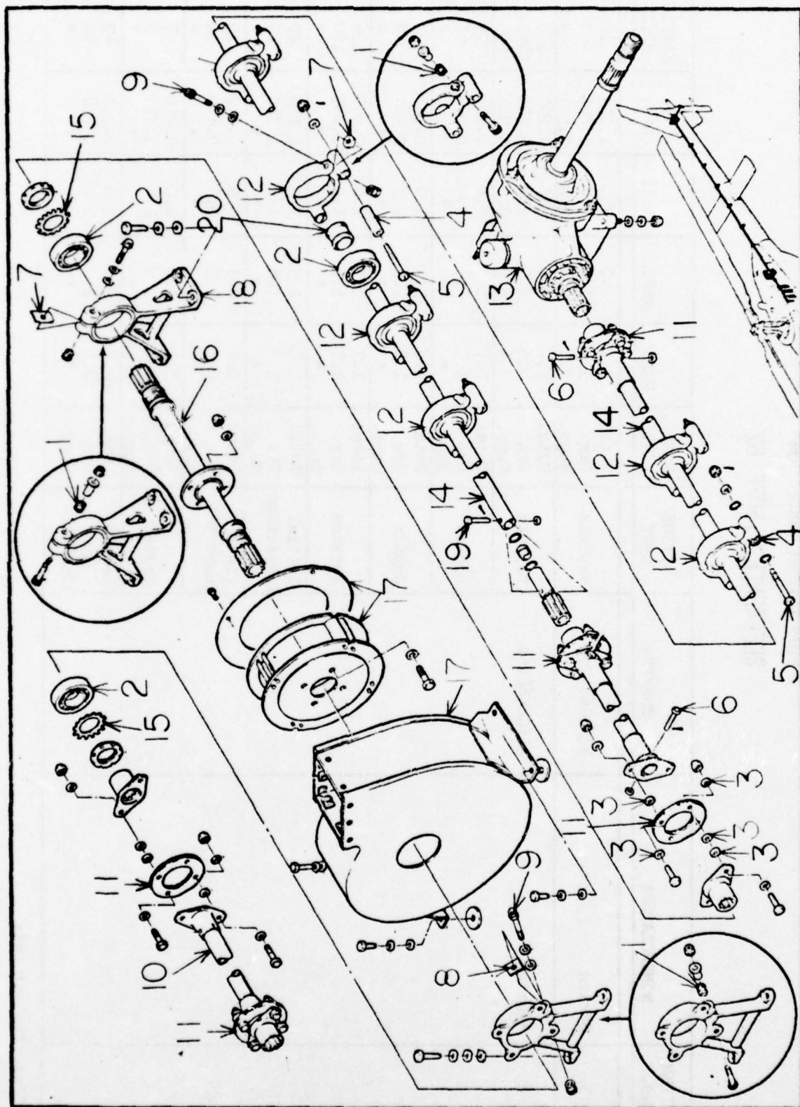
Figure 62 Tail Rotor Drive Shaft Installation
