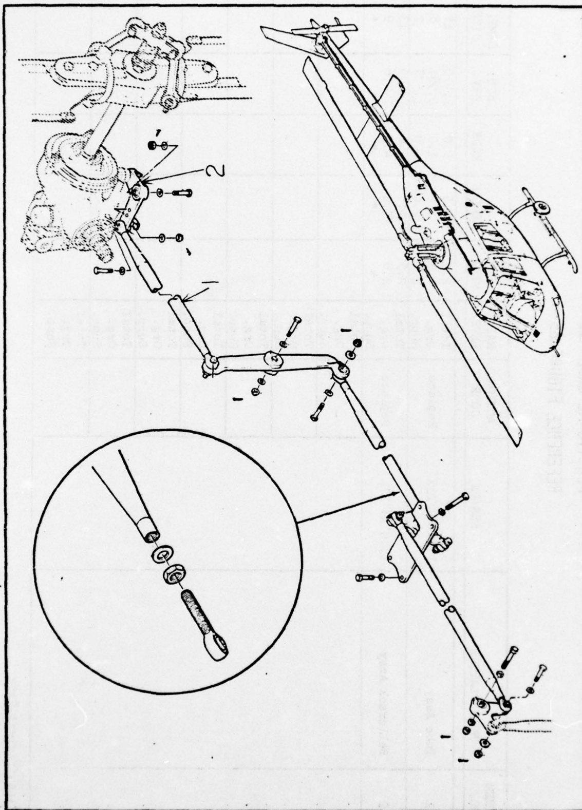
Figure 85 Antitorque System Controls Installation
