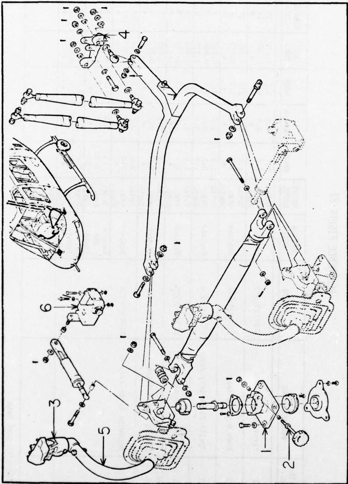
Figure 82 Cyclic Controls Installation
