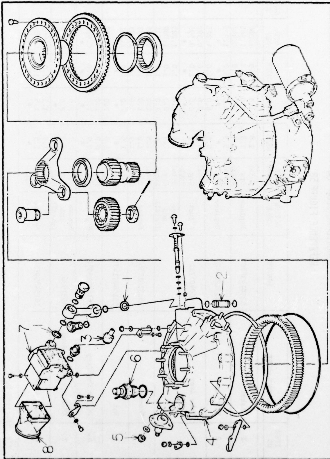
Figure 58 Transmission Assembly
