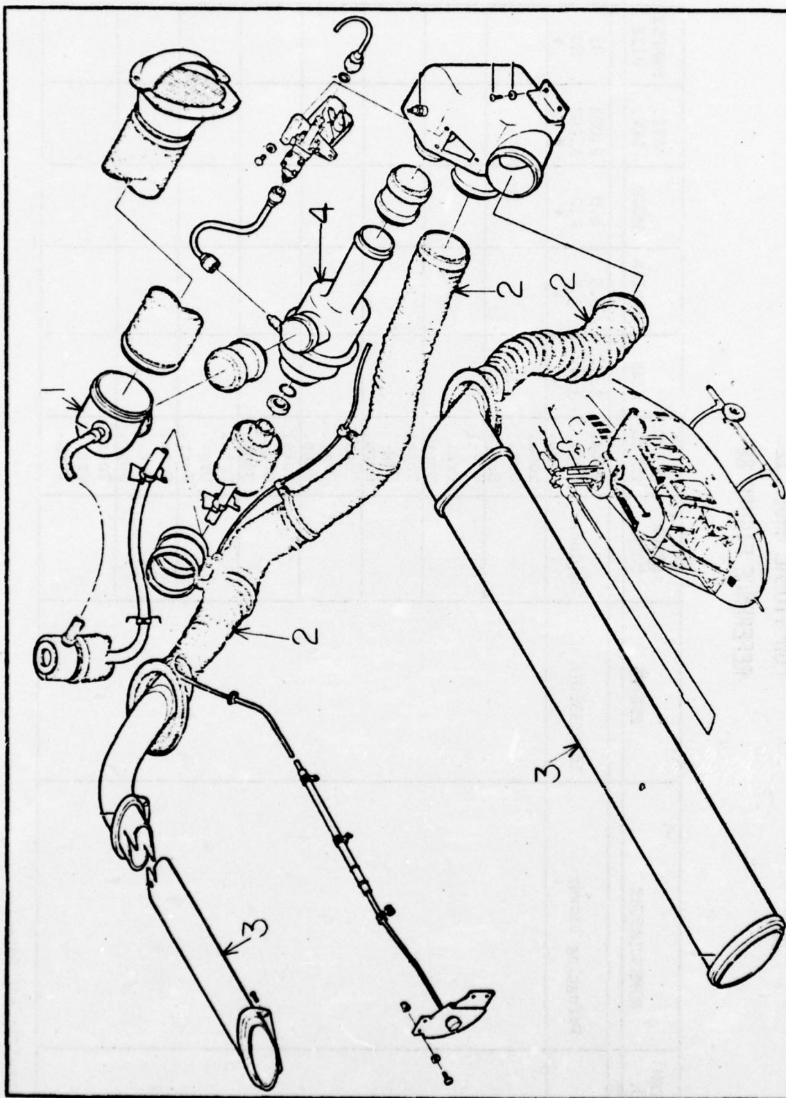
Figure 89 Bleed Air Heater Installation
