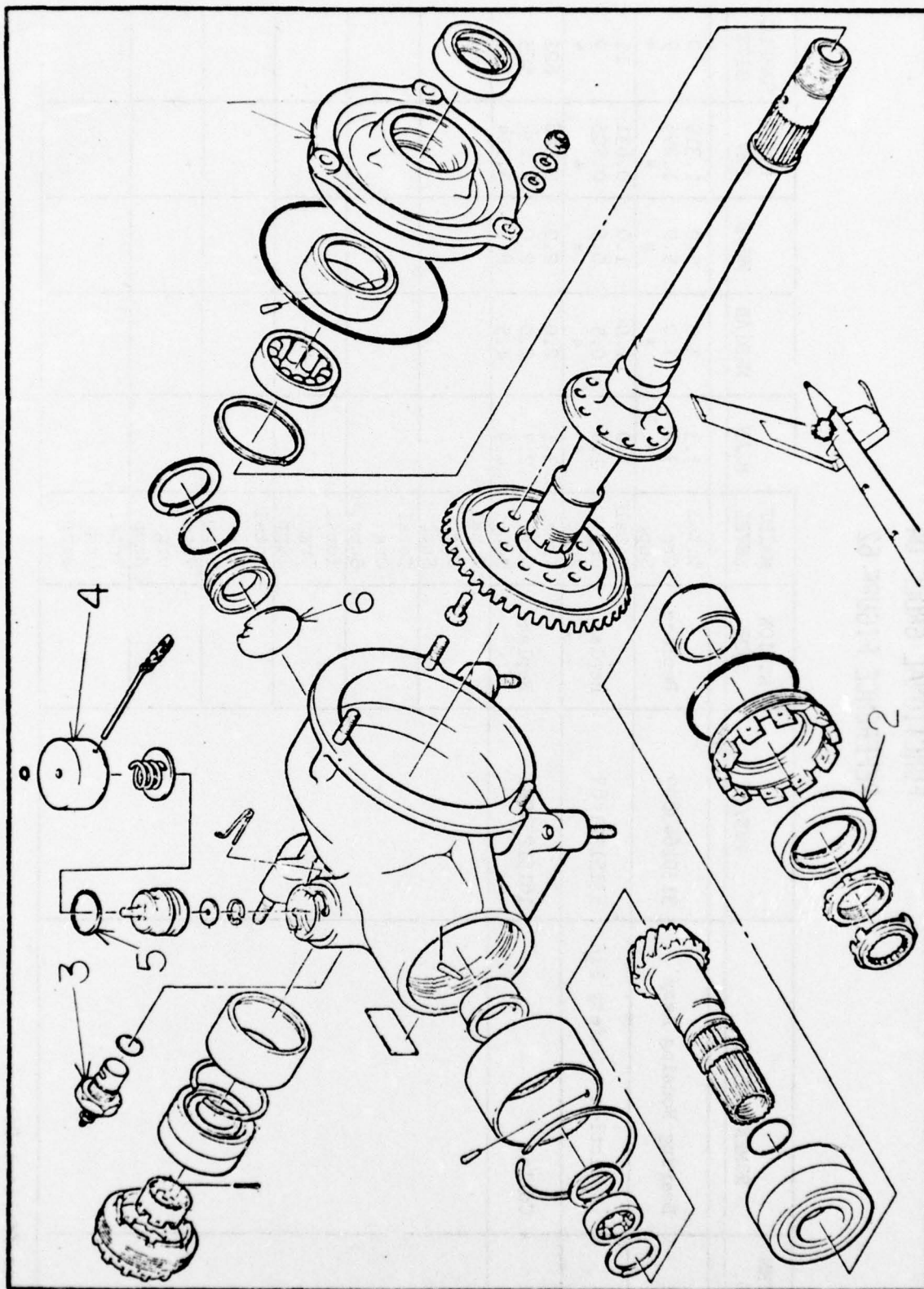
Figure 63 Tail Rotor Gear Box Assembly
