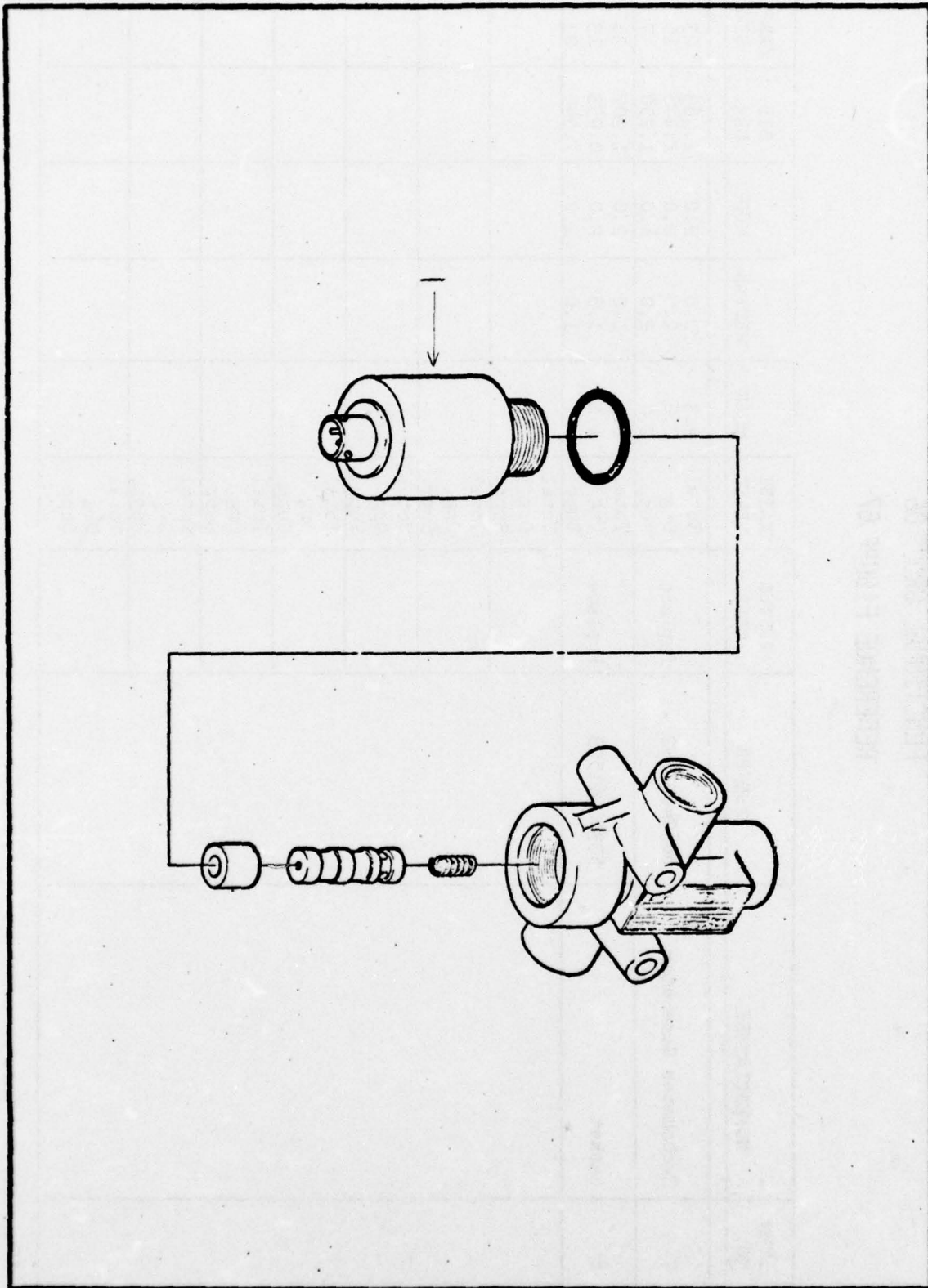
Figure 68 Solenoid Valve
