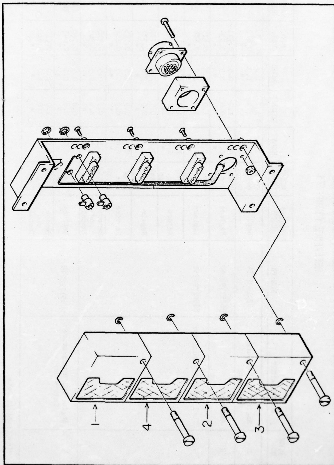
Figure 73 Engine Gage Unit
