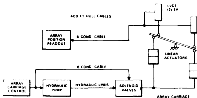
Figure 3. Array position control block diagram.
